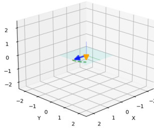
Step 1: Rotate 45° in xy-plane (bivector e_{12} )
