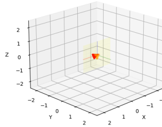
Step 2: Rotate 45° in xz-plane (bivector e_{13} )
