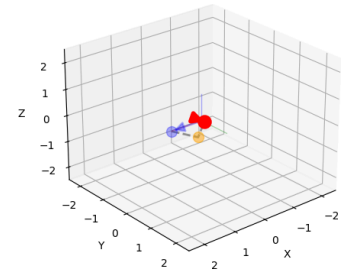
Combined Result R_{\text{combined}} = R_2 * R_1
