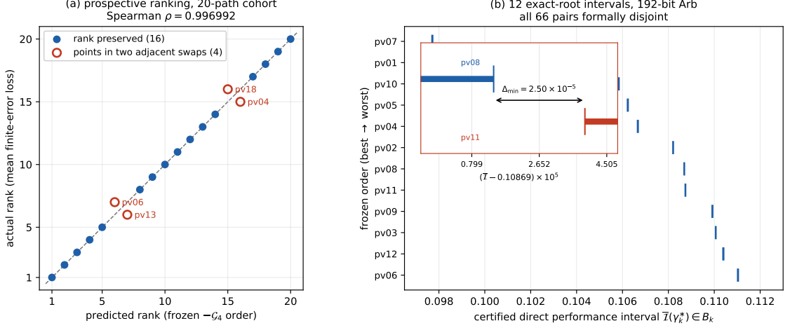
Figure 2: Direct visual evidence for the two claims in the title. (a) Prospective prediction: predicted versus actual ranks on the held-out twenty-path cohort. The frozen -\mathcal{G}_4 order reproduces the actual mean-loss ranking up to two adjacent transpositions (marked), giving Spearman \rho = 0.996992 . This panel reports prospective empirical evidence; it is not a certificate. (b) Exact-root certification: the twelve certified direct performance intervals B_k from 192-bit outward-rounded Arb propagation, drawn to scale in the frozen order. All 66 unordered pairs are formally disjoint; the tightest pair, pv08–pv11, has the certified margin \Delta_{\min} = 2.50 \times 10^{-5} of Corollary 3 (inset: magnification of that pair).
