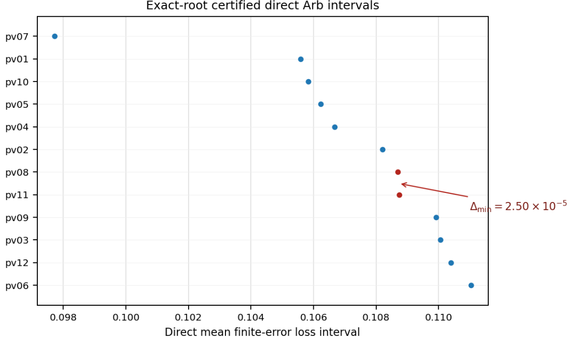
Figure 2: Direct visual evidence for the exact-root certification theorem. The prospective \mathcal{G}_4 result is reported only at threshold level in the text. This panel shows the exact-root certification: the twelve certified direct performance intervals B_k from 192-bit outward-rounded Arb propagation, drawn to scale in the frozen order. All 66 unordered pairs are formally disjoint; the tightest pair, pv08–pv11 (highlighted), has the certified margin \Delta_{\min} = 2.50 \times 10^{-5} of Corollary 1 (margin marked in the panel).
