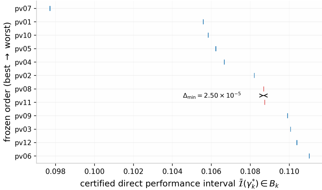
Figure 2: Direct visual evidence for the exact-root certification theorem. The prospective \mathcal{G}_4 result is reported only at threshold level in the text. This panel shows the exact-root certification: the twelve certified direct performance intervals B_k from 192-bit outward-rounded Arb propagation, drawn to scale in the frozen order. All 66 unordered pairs are formally disjoint; the tightest pair, pv08–pv11 (highlighted), has the certified margin \Delta_{\min} = 2.50 \times 10^{-5} of Corollary 1 (margin marked in the panel).
