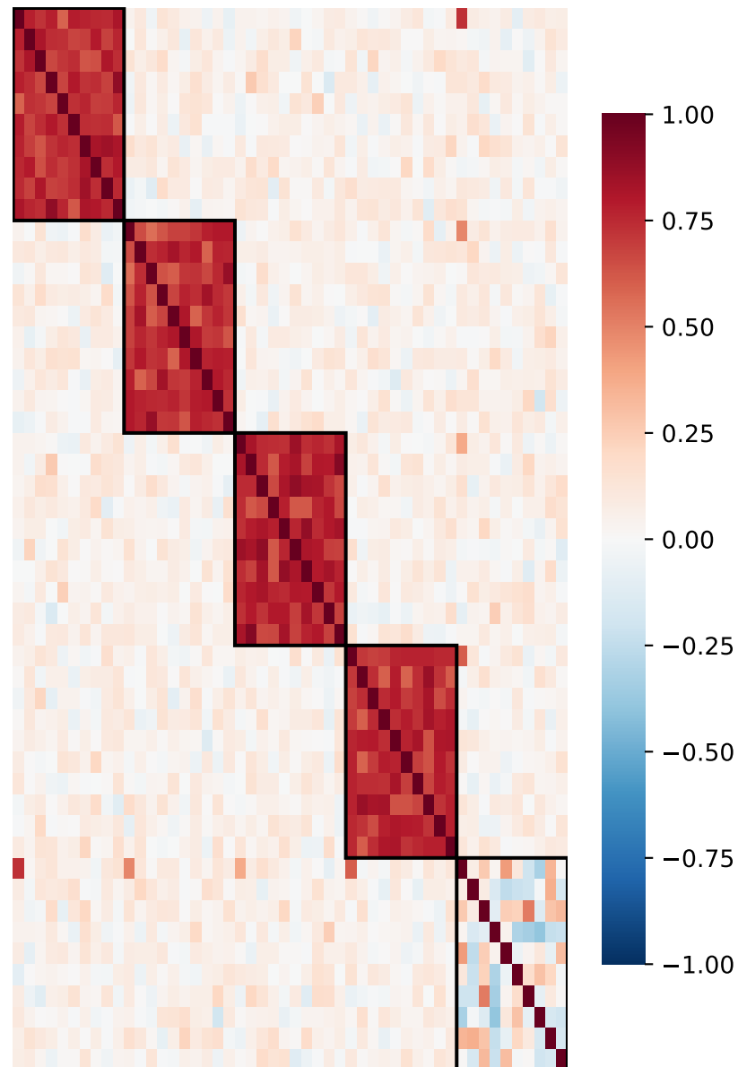
G_2 (Cancer)
