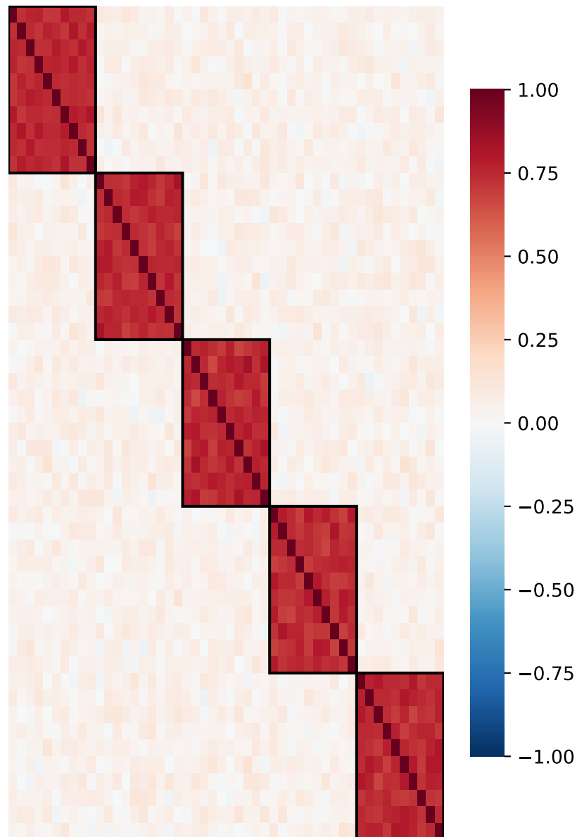
G_1 (Normal)
