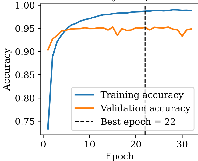
Accuracy vs Epoch
