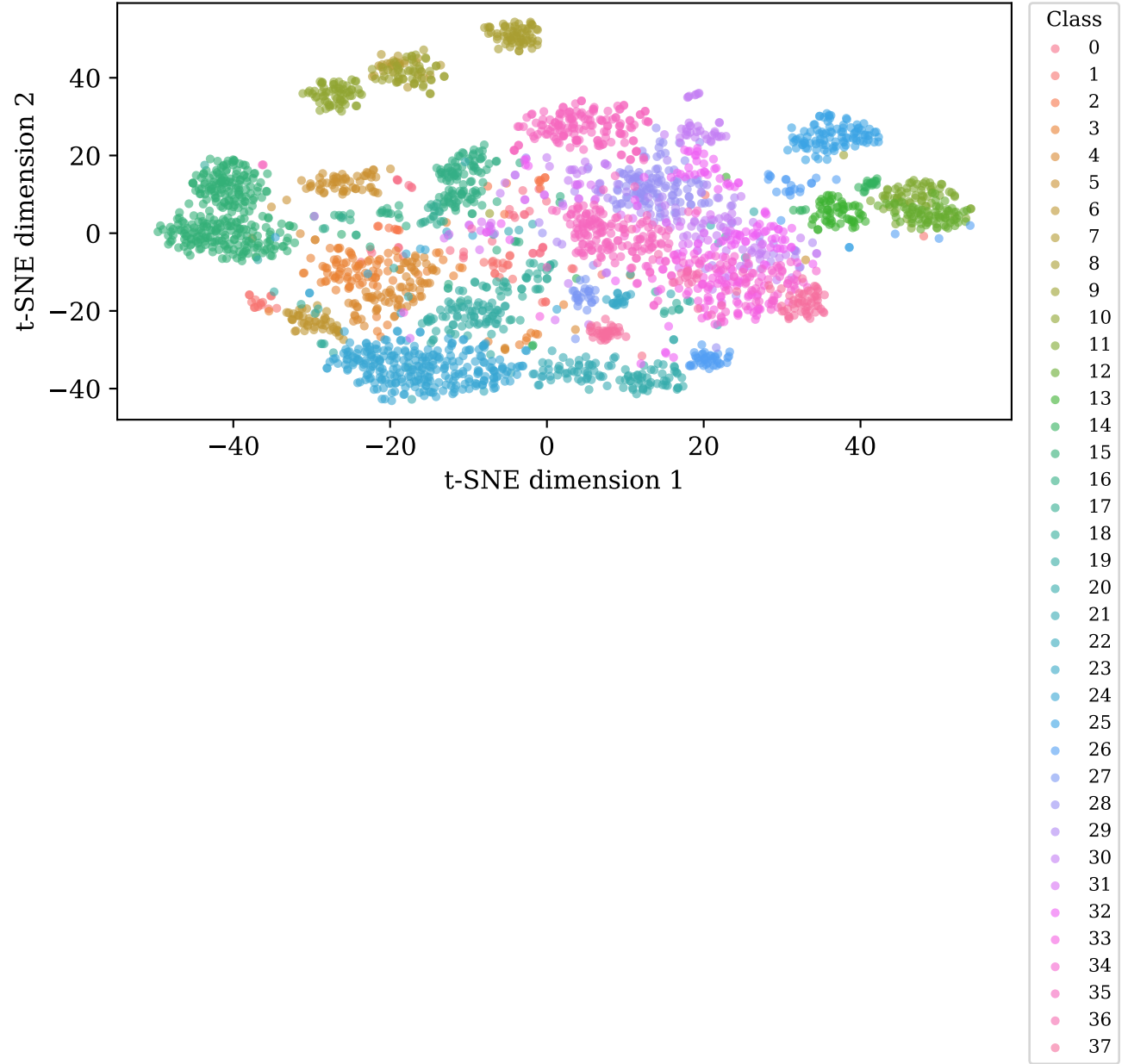
t-SNE projection of the 4608-d fused CNN feature space (PlantVillage test set)
