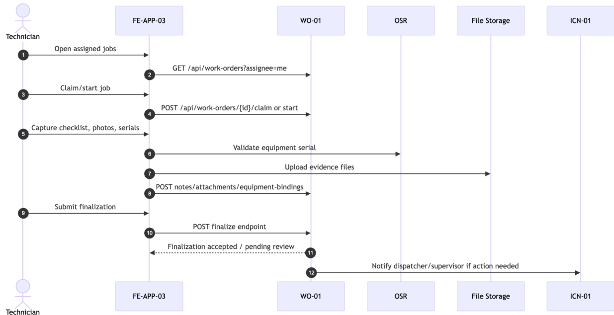
Figure 3 - Work order execution flow
