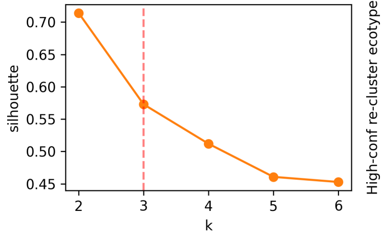
Silhouette
