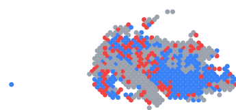
A pDMG Sample-1 577 spots same-neighbor 0.540 vs null 0.358, P = 0.001
