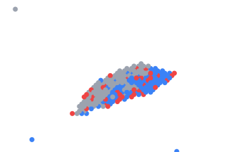
C pDMG Sample-3 217 spots same-neighbor 0.562 vs null 0.370, P = 0.001
