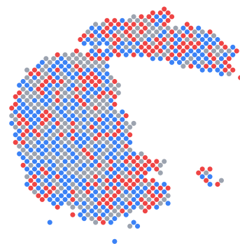
B pDMG Sample-2 856 spots same-neighbor 0.357 vs null 0.338, P = 0.019
