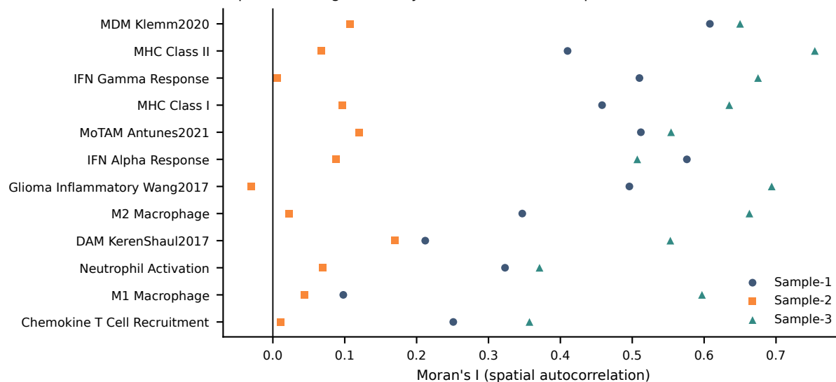
D Immune programs are spatially structured, not randomly distributed top 12 of 24 signatures by mean Moran's I; 999-permutation test
