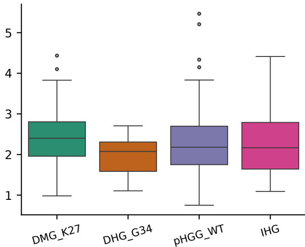
TIS by cohort H=14 p=3e-03 \epsilon^2=0.03
