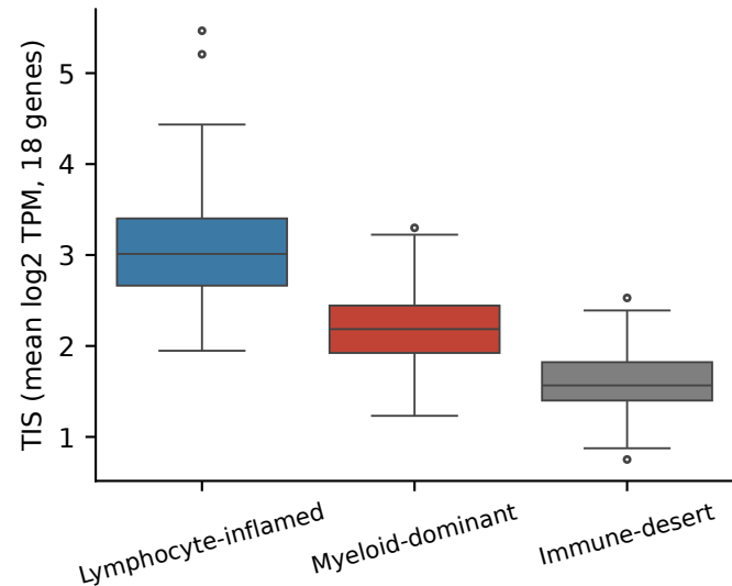
TIS by ecotype H=216 p=1e-47 \epsilon^2=0.62
