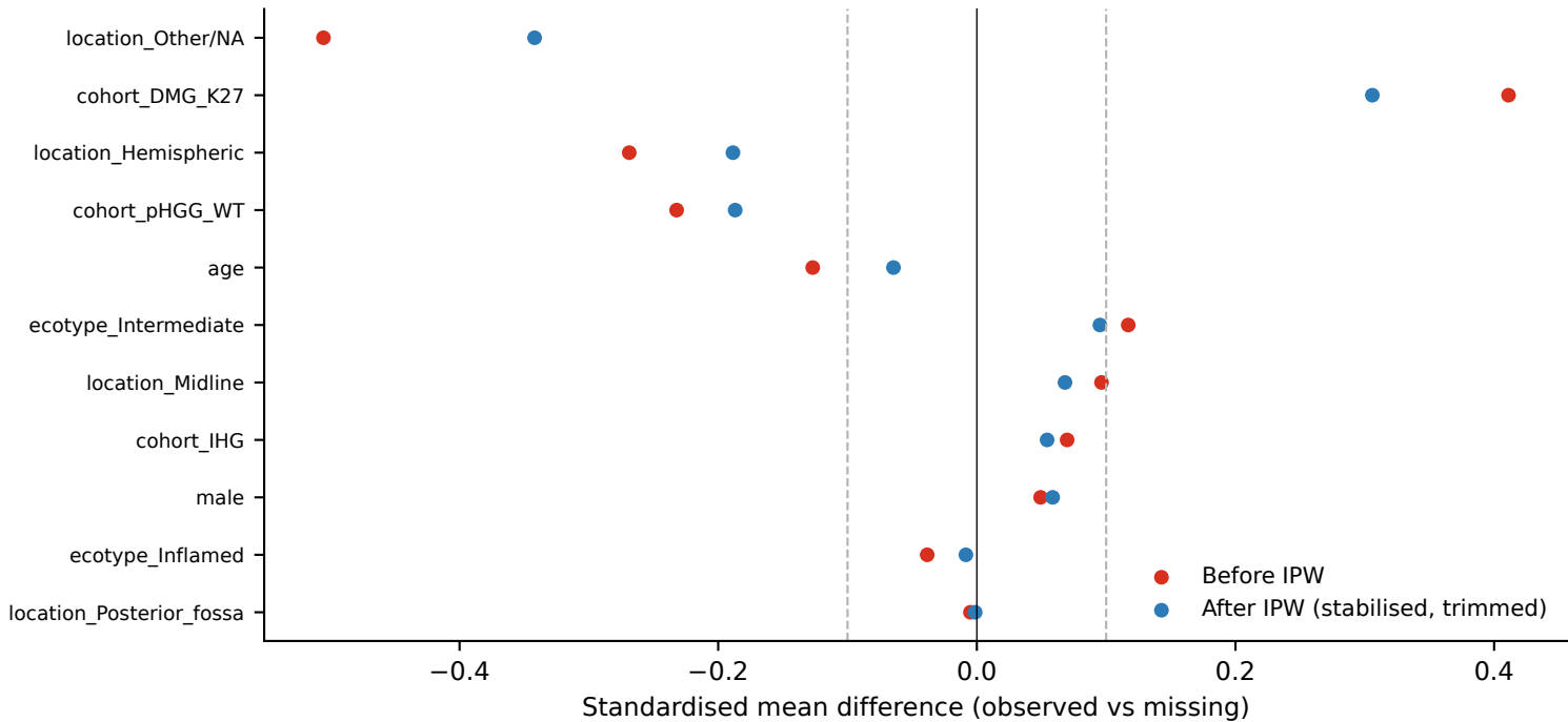
Love plot — covariate balance before vs after IPW ( |SMD| > 0.1 : 6 \rightarrow 4)
