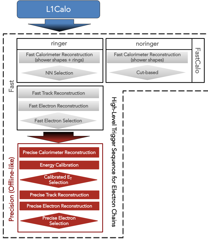
Figure 1: This figure presents the sequence of algorithms used to select electron candidates at the High Level Trigger stage. Differences between the original baseline (no-ringer) and new (ringer) electron triggers lie in the first step, called FastCalo. Grey blocks represent algorithms in the fast stage, and red blocks represent precision-step algorithms.
