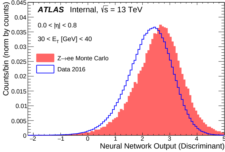
Figure 5: Differences between simulation samples (filled histogram) and collision data (empty histogram) obtained in 2016 Z \rightarrow e^+e^- tag-and-probe for one region of the phase space. The comparison is made between the normalized distributions of the output of the neural network (the discriminant) obtained for these two cases. The shift in discriminant value between simulation and collision data is caused by differences between the simulation and data rings used as input to the model.
