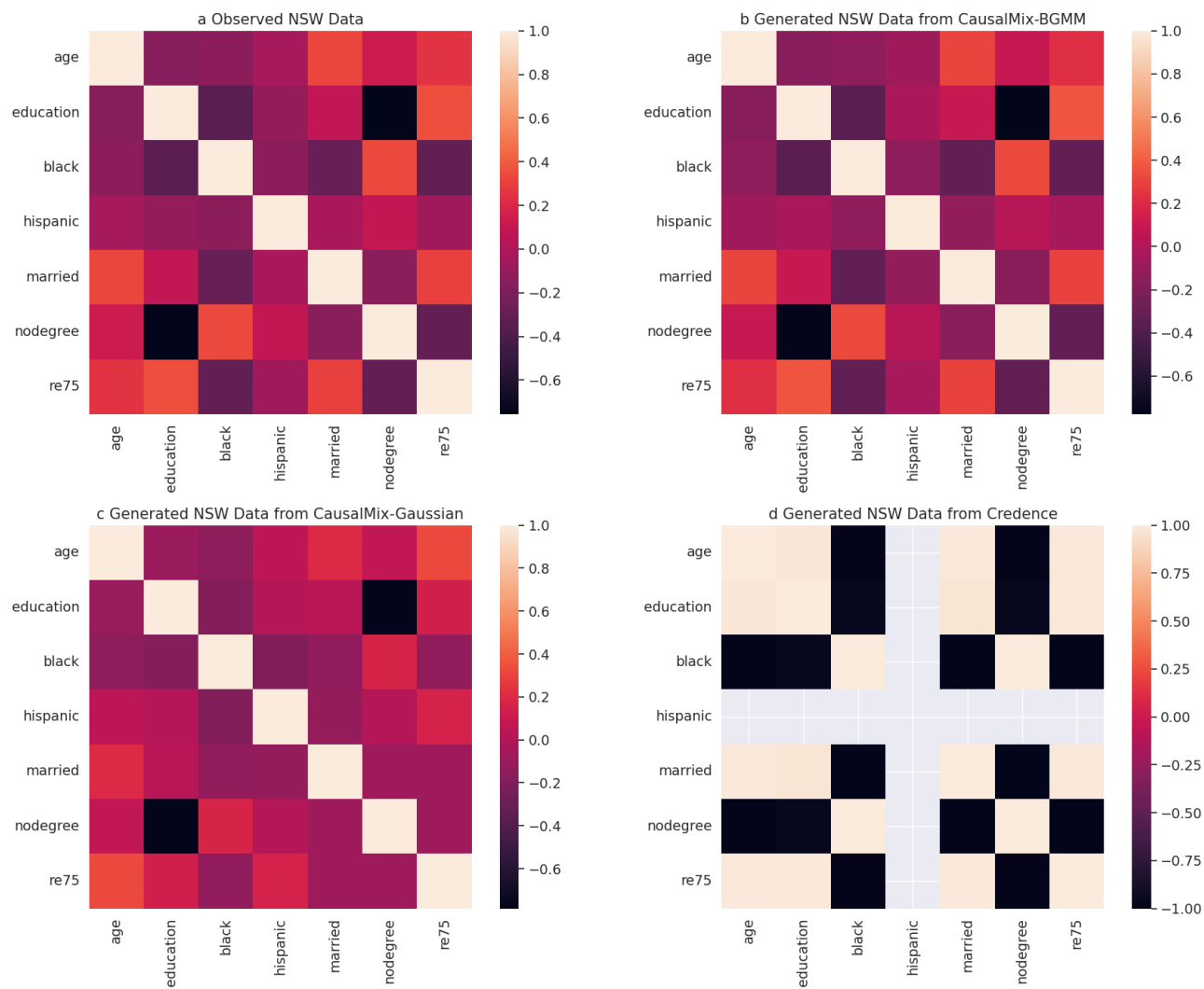
Figure 2. Correlation structure comparison: real vs. generated data (CausalMix vs. Credence). Empty cells were produced in the panel (d) because of constant values.
