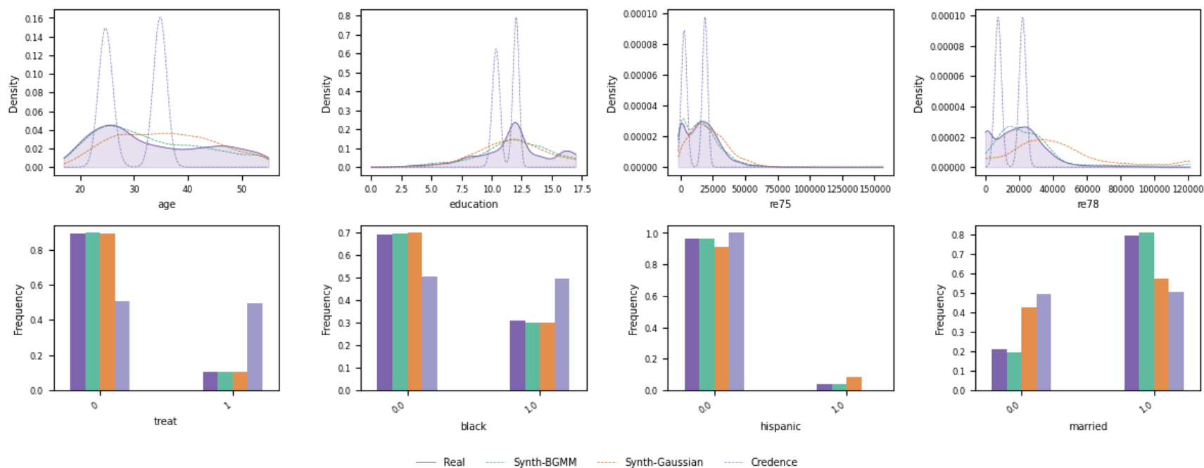
Figure 1. Marginal distribution comparison (real vs. synthetic data). Colors denote data sources: real data (blue), CausalMix-BGMM (green), CausalMix-Gaussian (orange), and Credence (purple).
