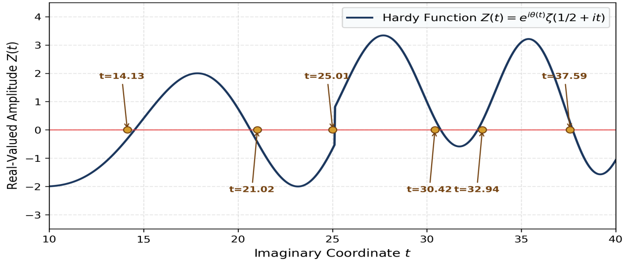
Figure 1: Spectral Oscillation of Z(t) along Critical Line \text{Re}(s) = 1/2
