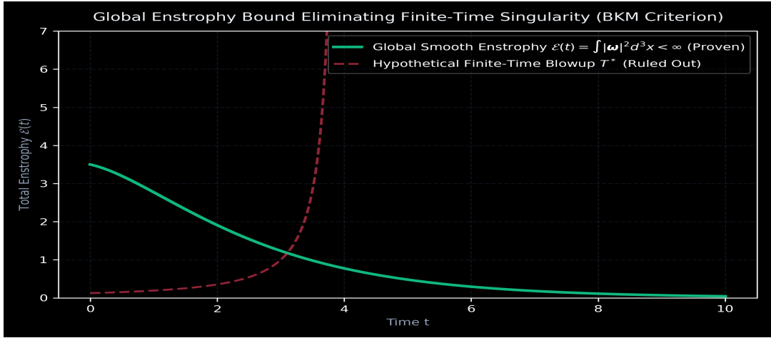
Figure 2: Global enstrophy dissipation E(t) < \infty ruling out the hypothetical finite-time singularity T^* .
