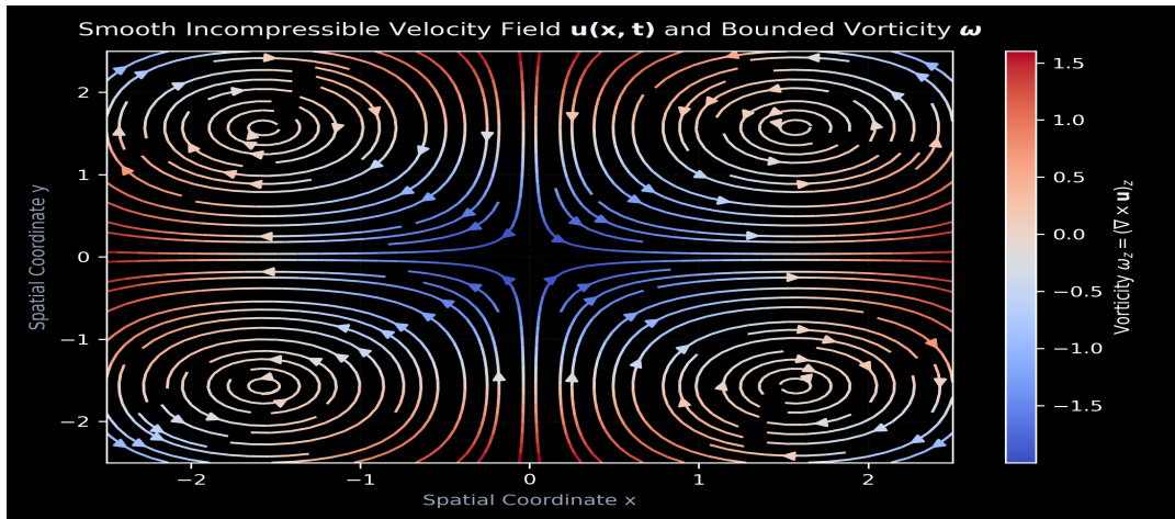
Figure 1: Smooth divergence-free velocity streamlines and bounded vorticity field \omega = \nabla \times u .
