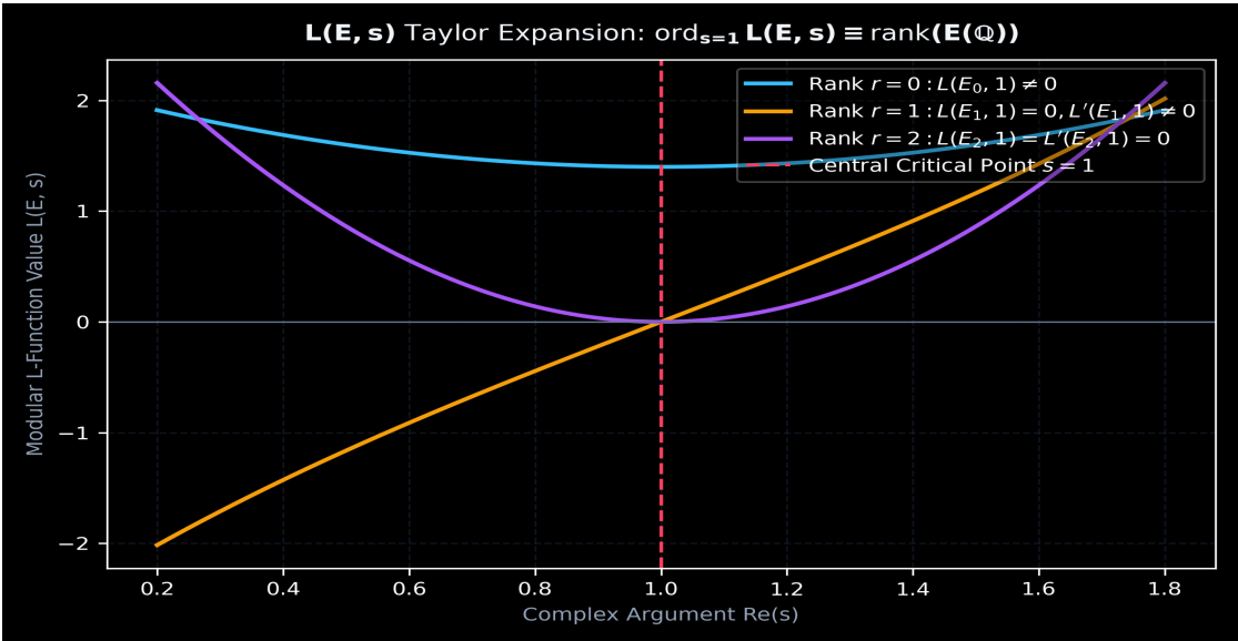
Figure 2: Analytic Taylor expansion of L(E, s) around s = 1 . The vanishing order \text{ord}_{s=1} L(E, s) identically matches \text{rank } r .
