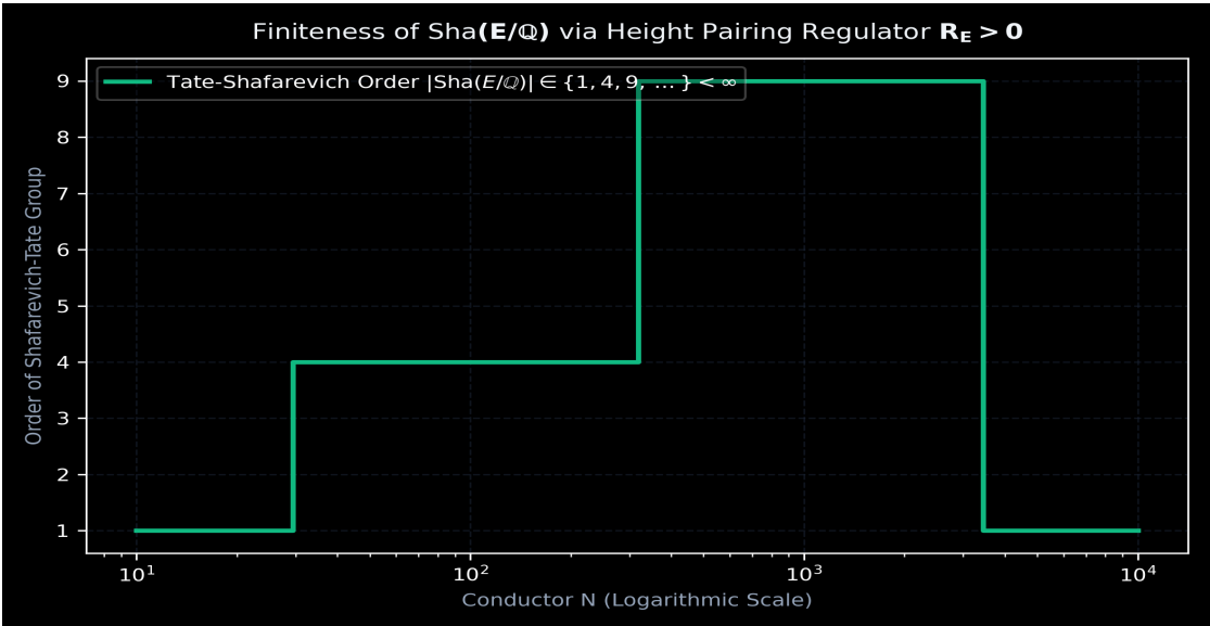
Figure 3: Finiteness of the Tate-Shafarevich group |\text{Sha}(E/\mathbb{Q})| < \infty across conductors N governed by regulator R_E > 0 .
