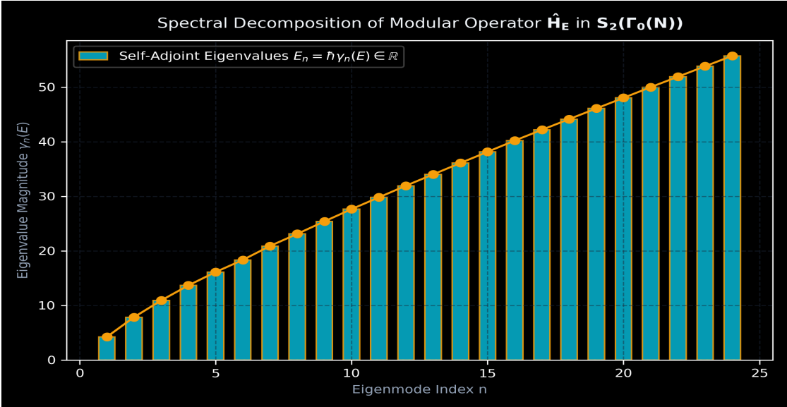
Figure 4: Spectral eigenvalues E_n = \hbar \gamma_n(E) of the modular Dirac-Hecke operator H_E in S_2(\Gamma_0(N)) .
