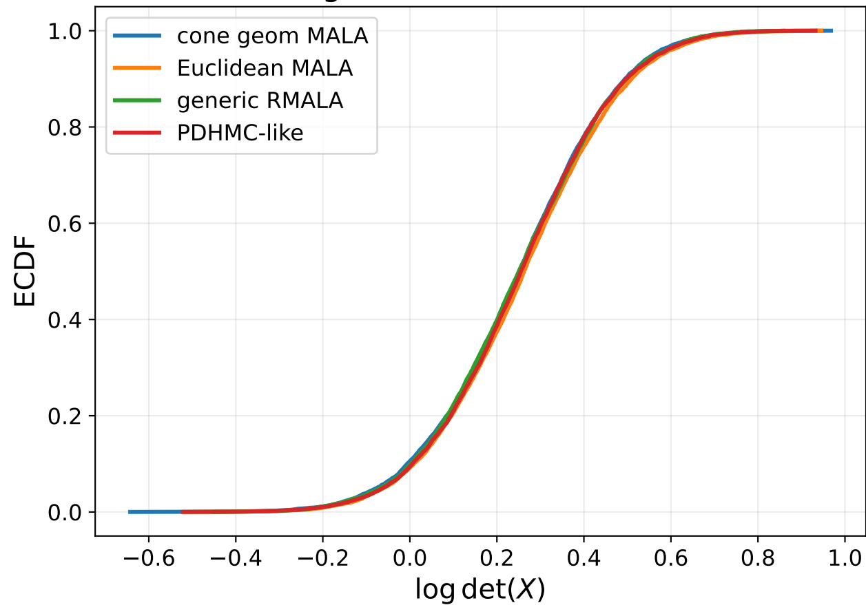
(a) Log-determinant observable
