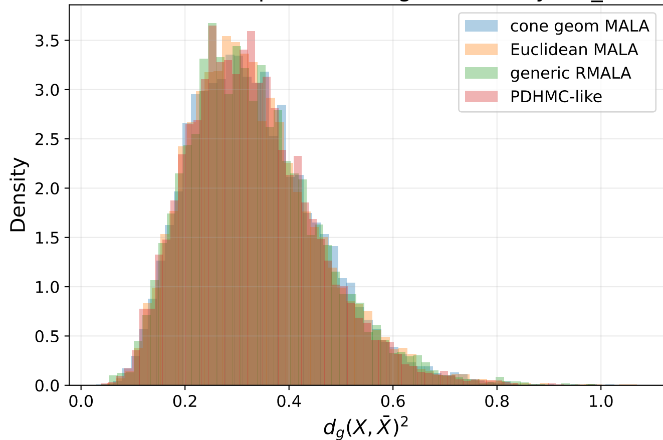
Cross-method pooled histogram overlay: d_2\_bar
