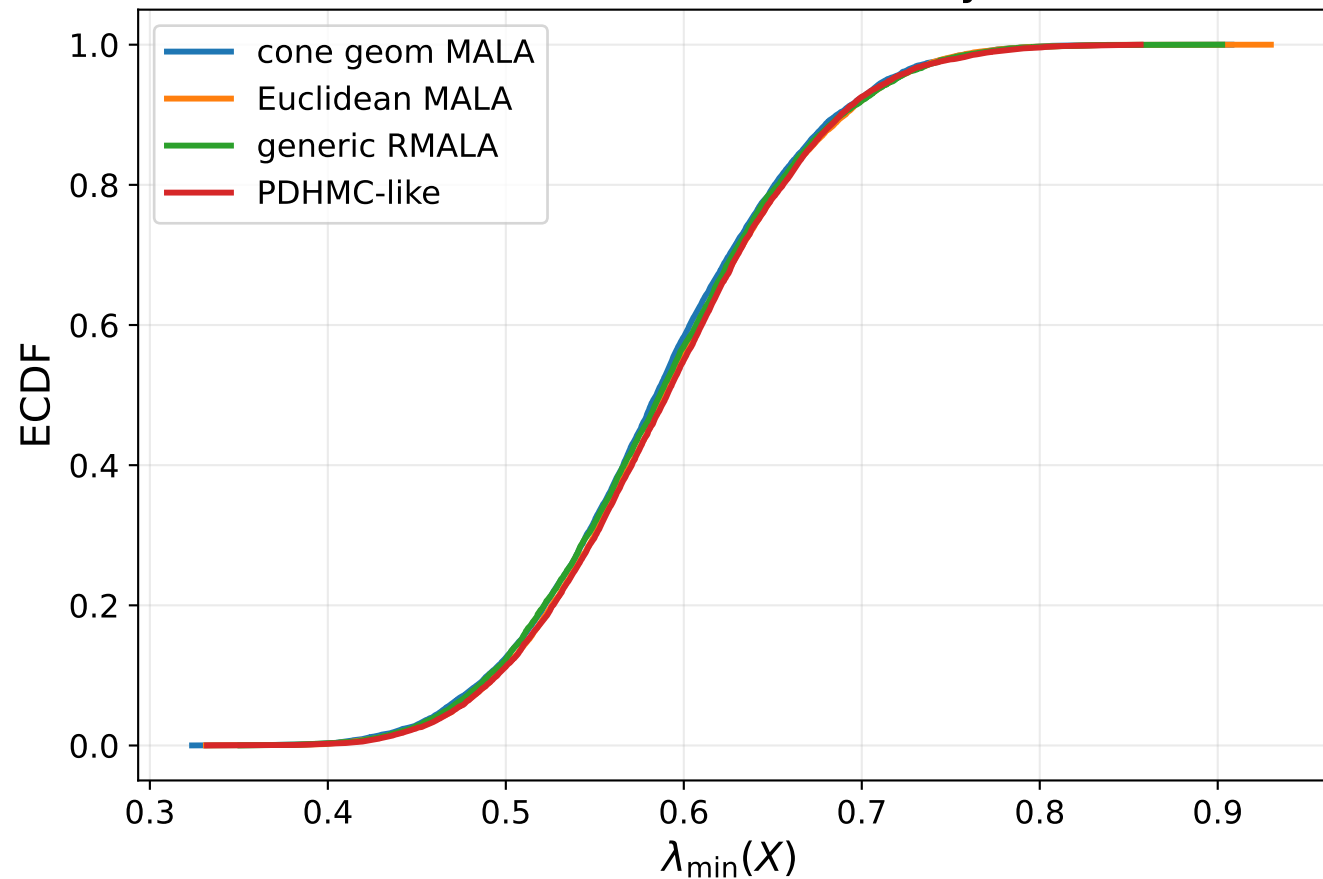
Cross-method ECDF overlay: \lambda_{\min}
