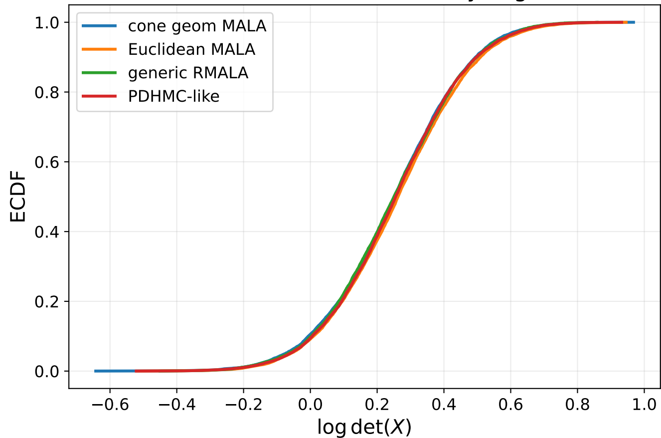
Cross-method ECDF overlay: logdet
