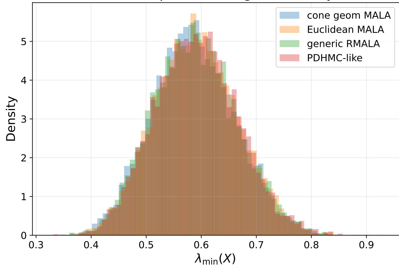
Cross-method pooled histogram overlay: \lambda_{\min}
