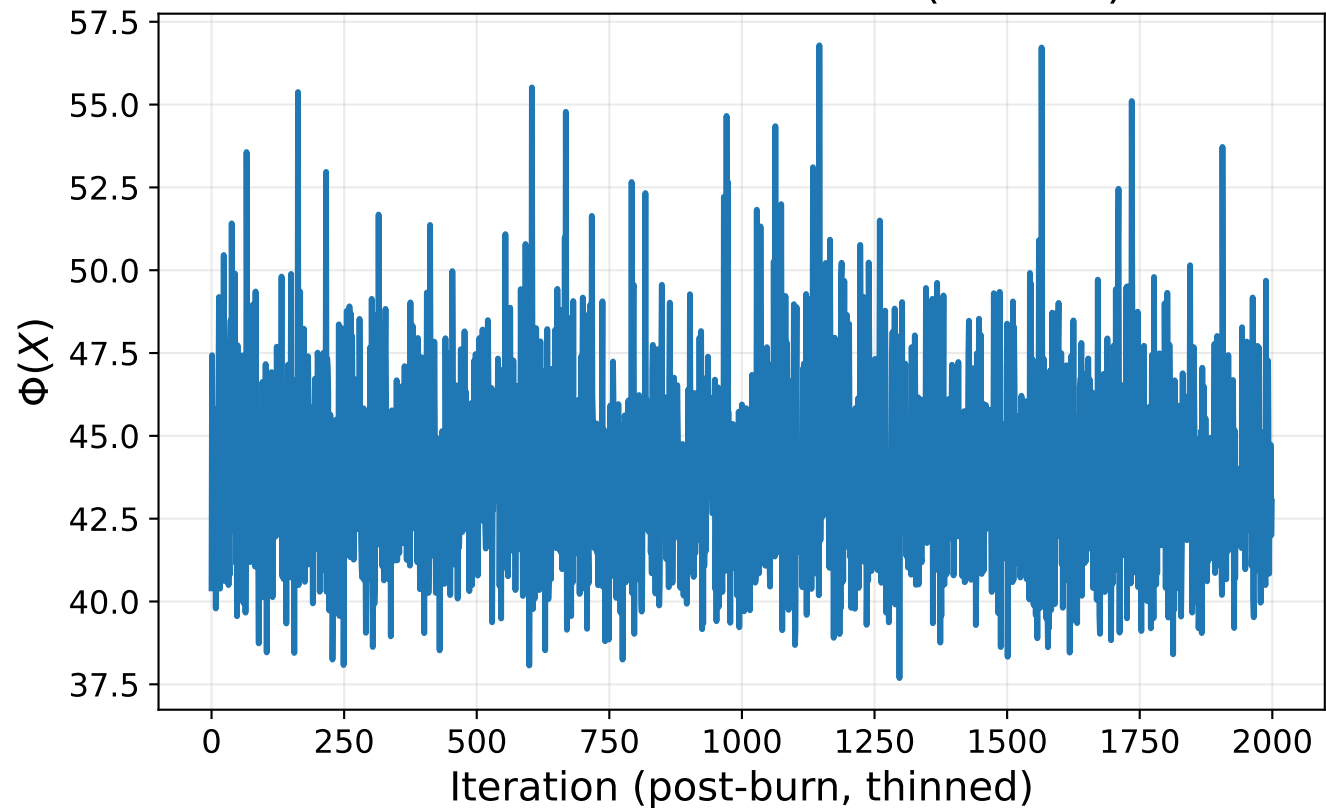
PDHMC-like: trace of \Phi (chain 0)
