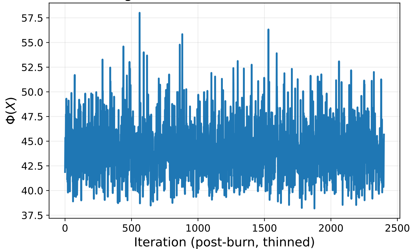
cone geom MALA: trace of \Phi (chain 0)
