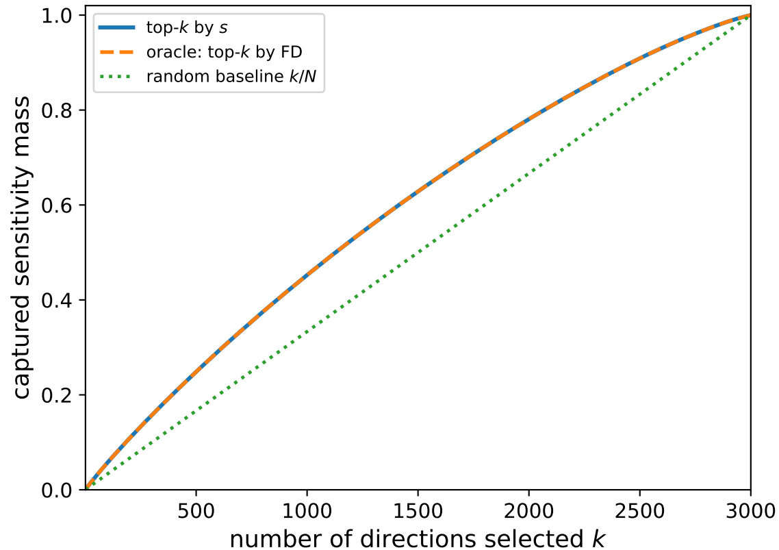
Panel B. Ranking / capture (PSD, d = 5 )
