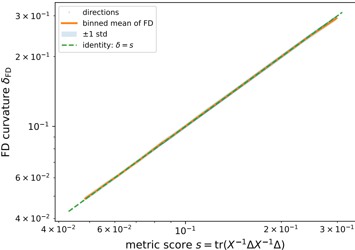
Panel A. Calibration (PSD, d = 5 )
