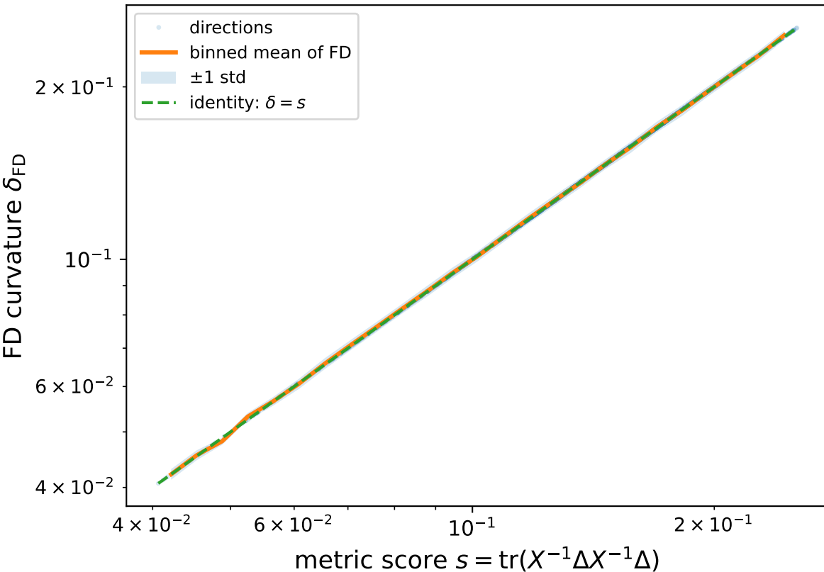
Panel A. Calibration (PSD, d = 3 )
