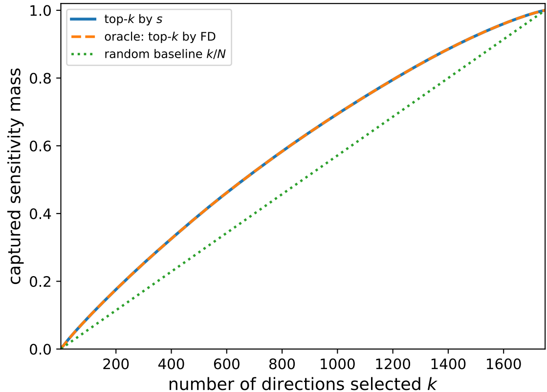
Panel B. Ranking / capture (PSD, d = 3 )
