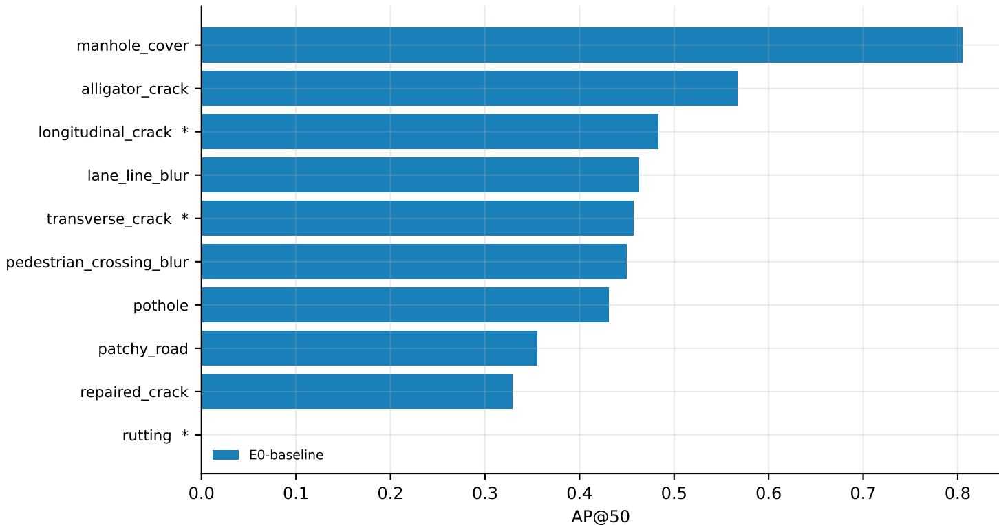
Per-class AP@50
