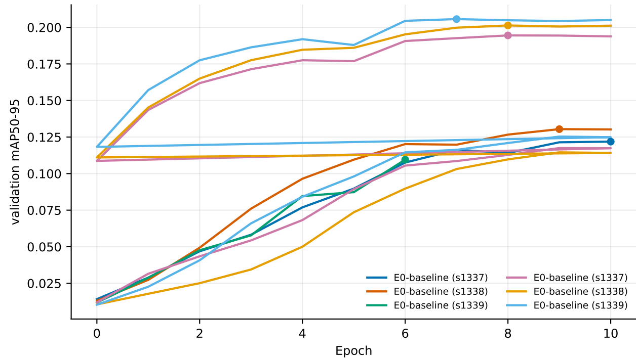
Training progress (dots mark each run's best epoch)
