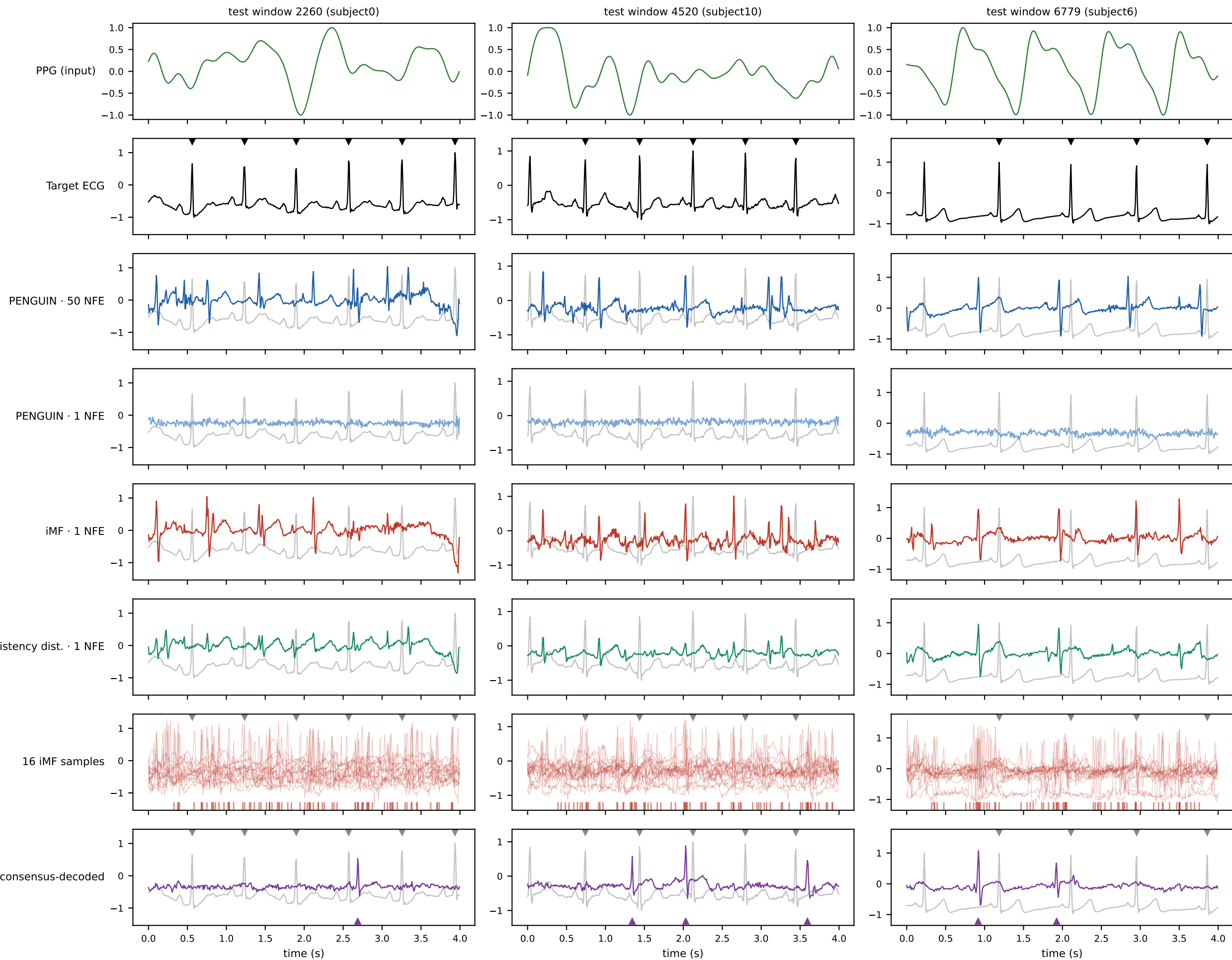
PPG-DaLiA — same test windows for every model; grey = target, ▼ = target R peaks, ▲ = consensus events, | = sample votes
