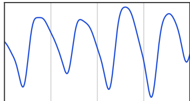
PPG-DaLiA
