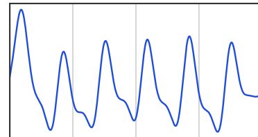
MIMIC-BP
