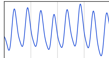
UCI-BP
