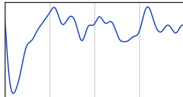
WildPPG
