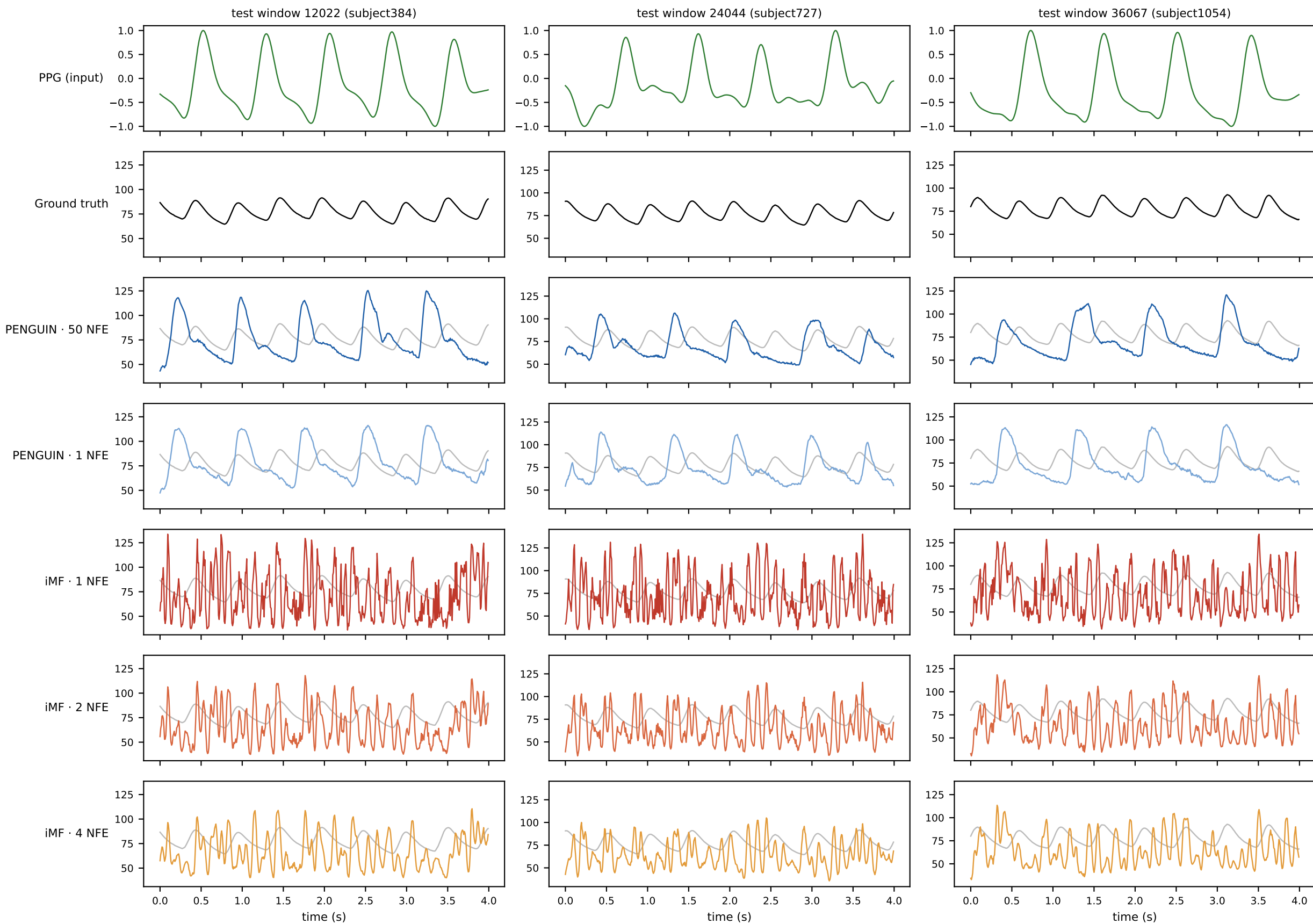
MIMIC-BP (ABP, target unit mmHg) — same test windows, noise seed 0, grey = ground truth
