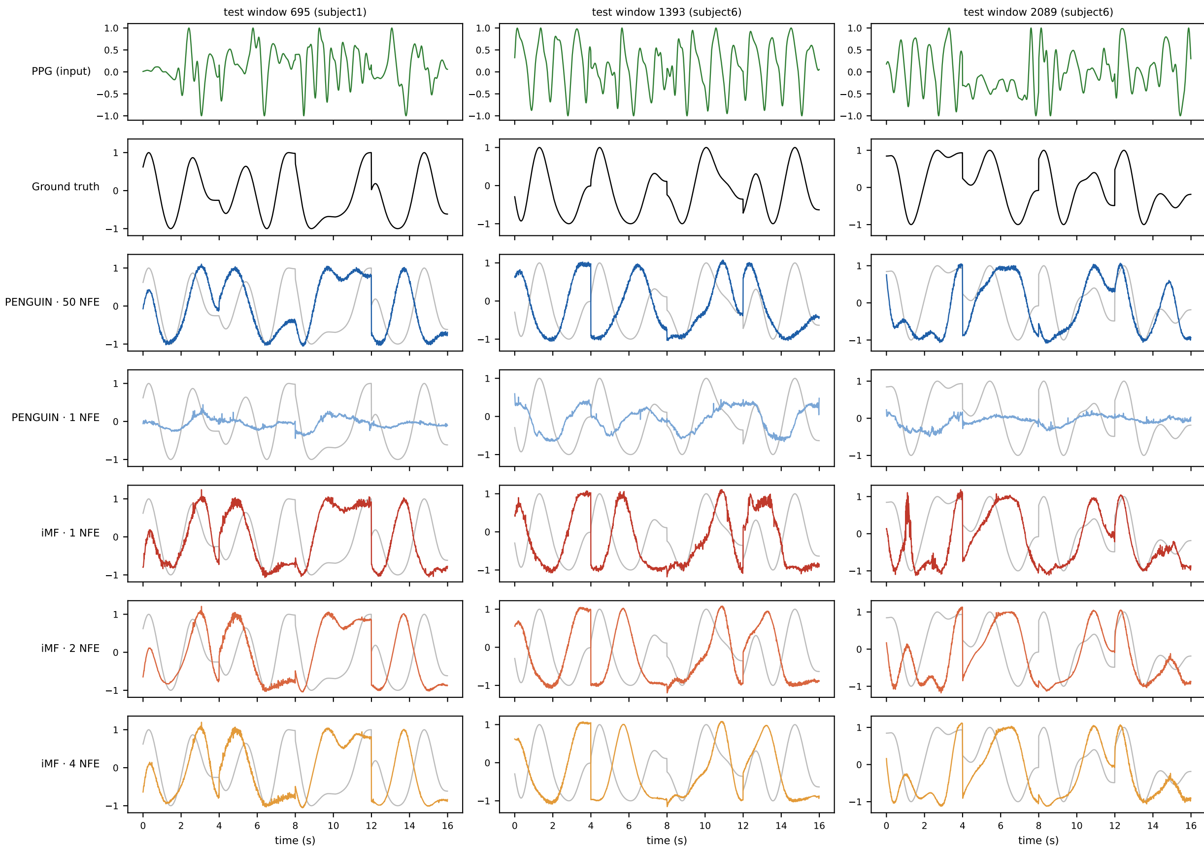
WESAD (Resp, target unit a.u.) — same test windows, noise seed 0, grey = ground truth
