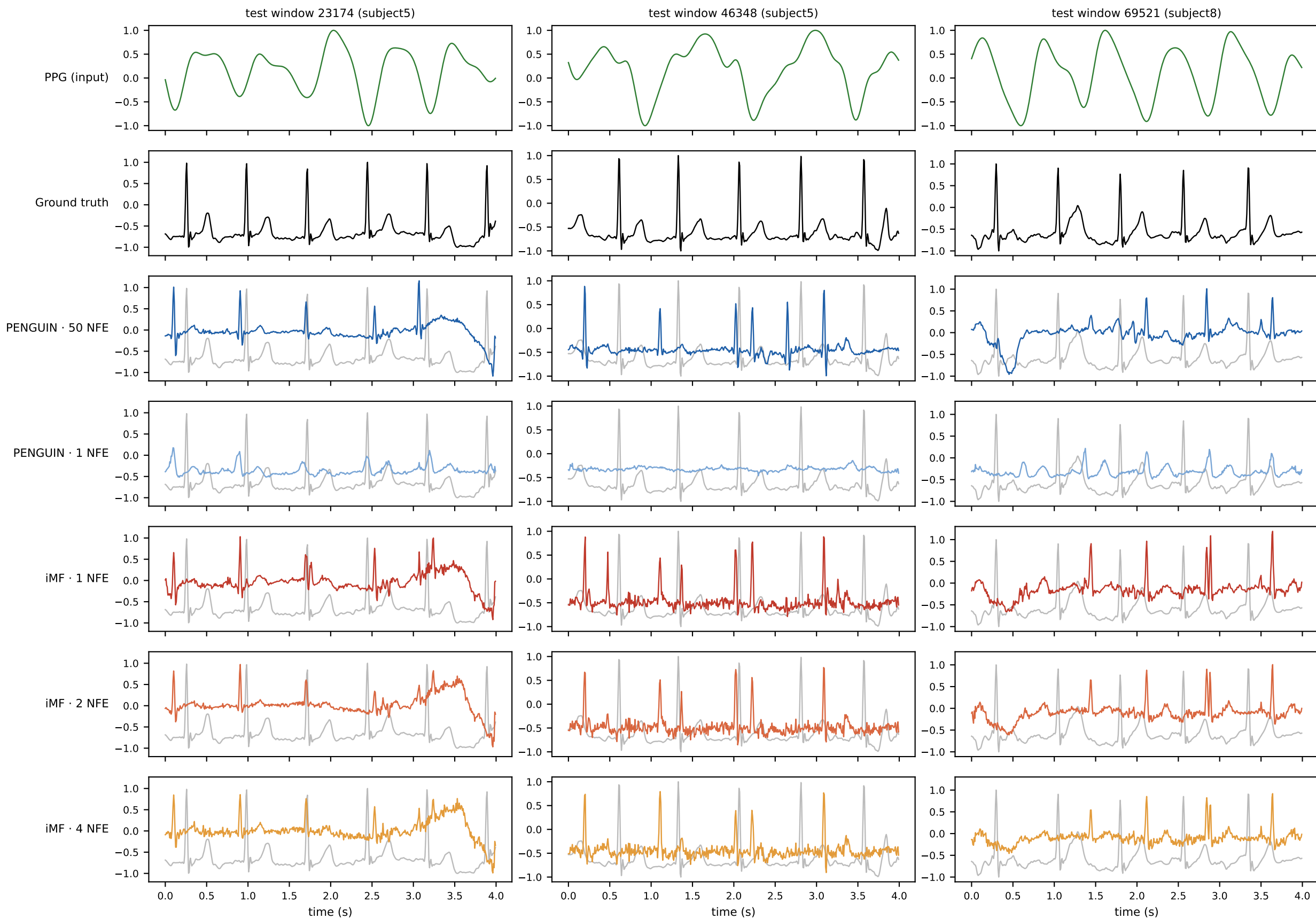
WildPPG (ECG, target unit a.u.) — same test windows, noise seed 0, grey = ground truth
