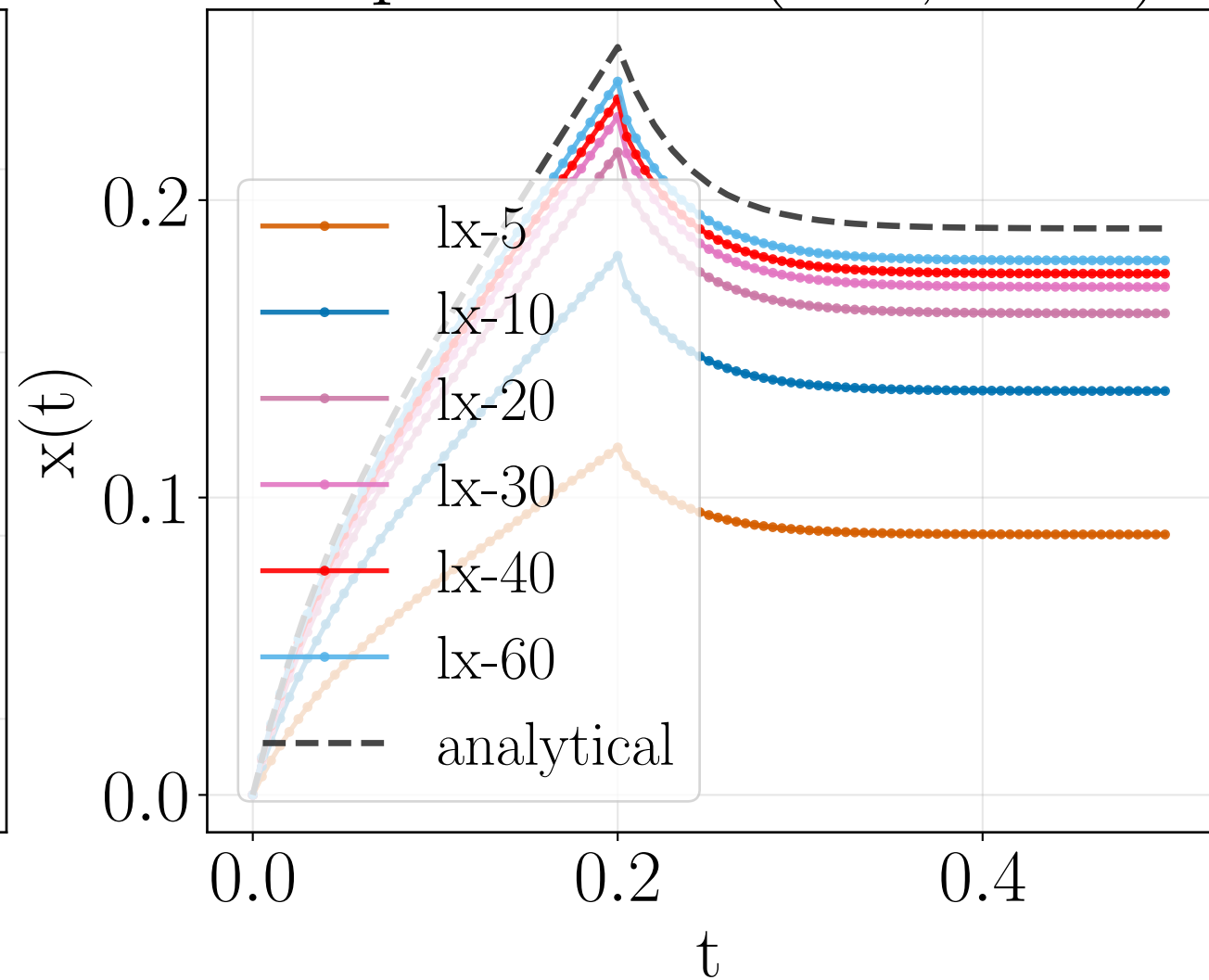
Displacement (raw, col 2)
