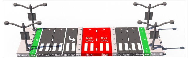
A completed model — center-running BRT lanes between two-way general purpose traffic, with protected bike lanes behind each curb.
