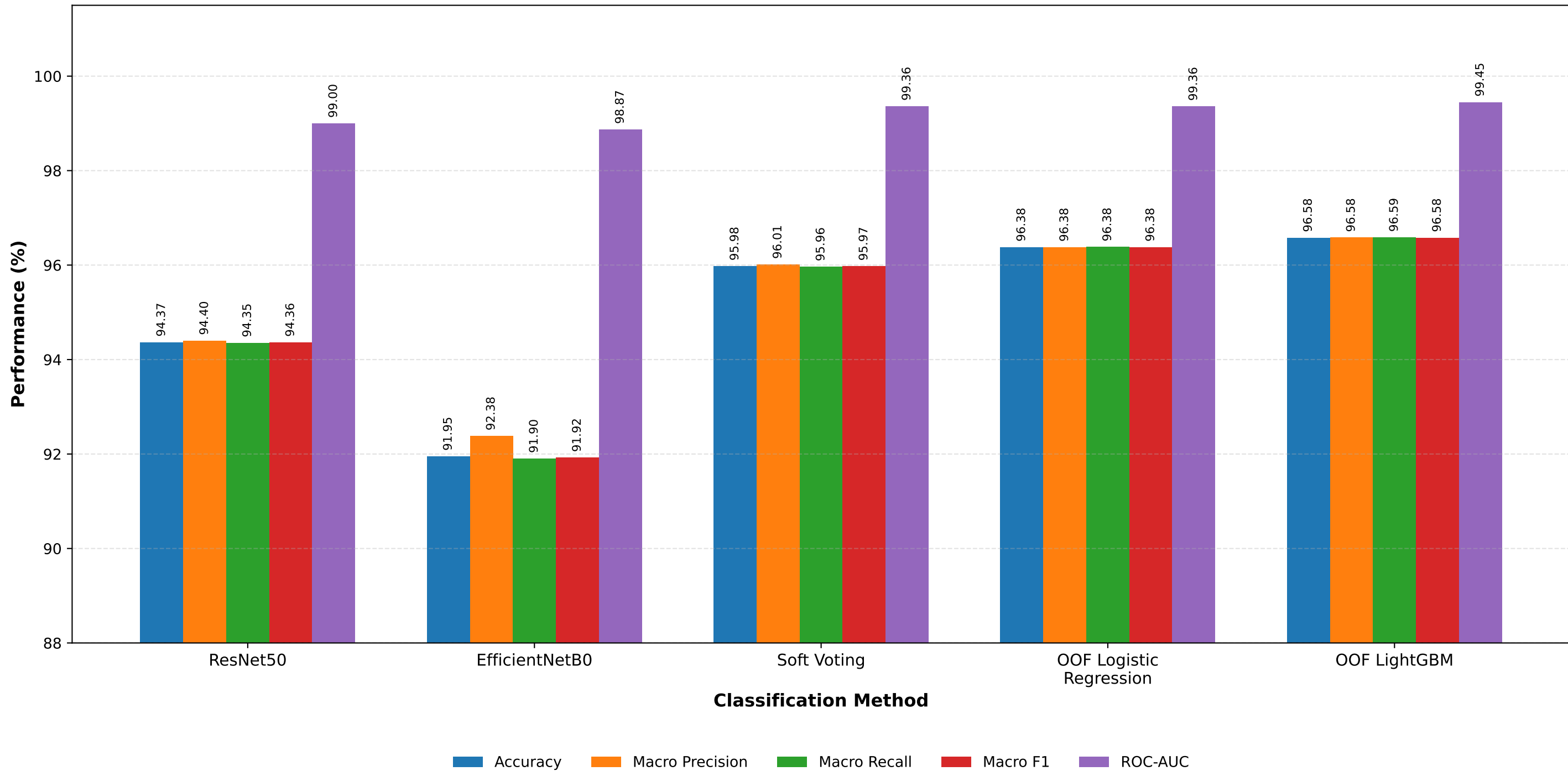
Performance Comparison of CT Base Models and OOF Ensemble Methods
