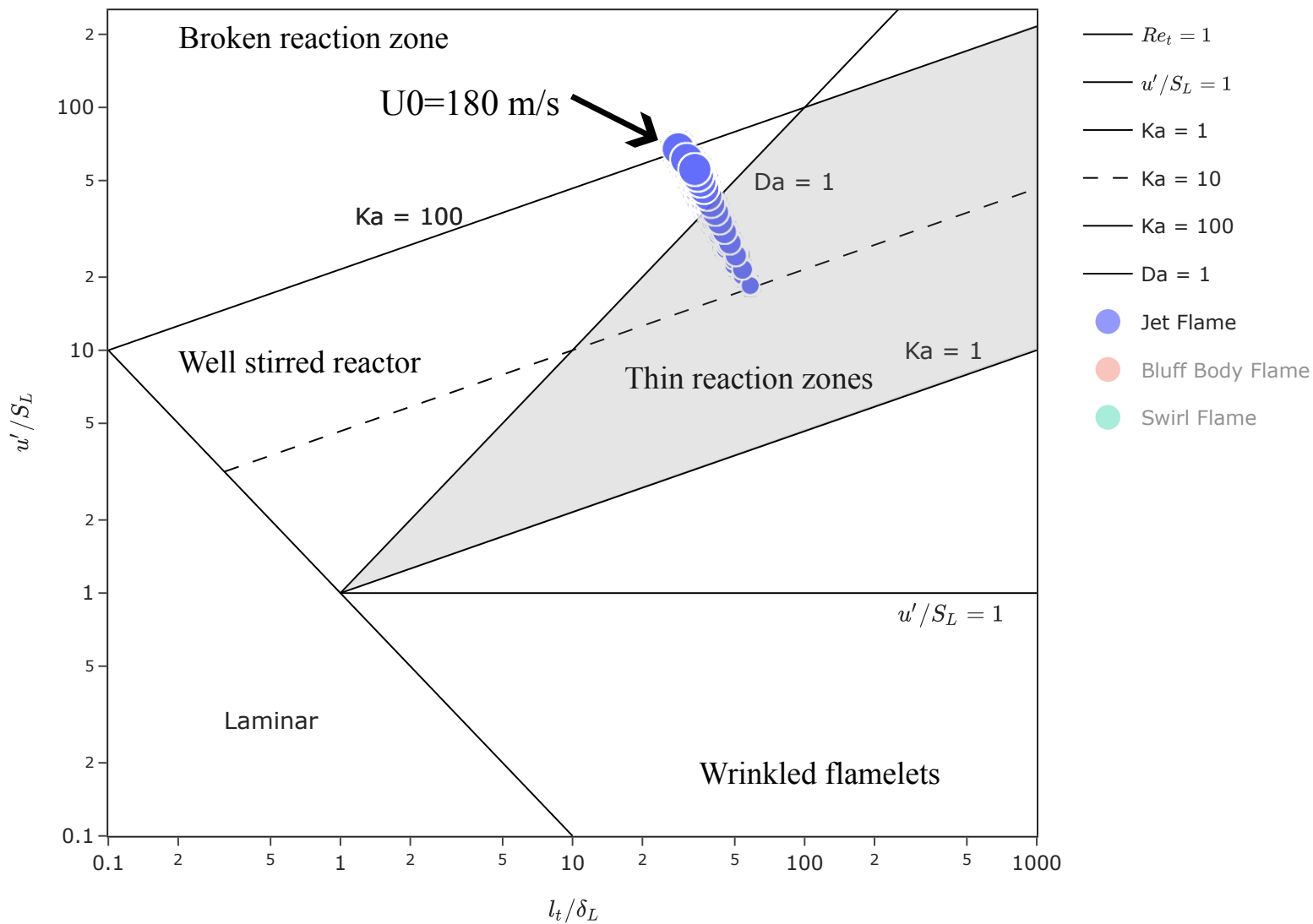
Borghi Diagram
