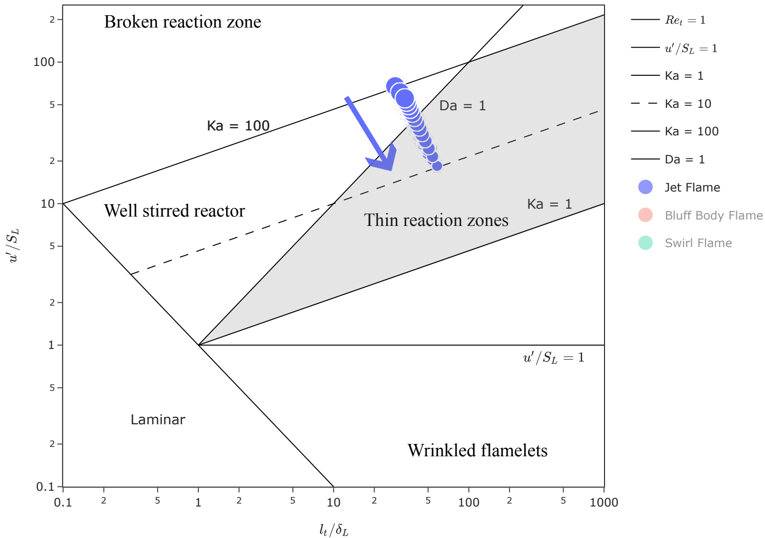
Borghi Diagram
