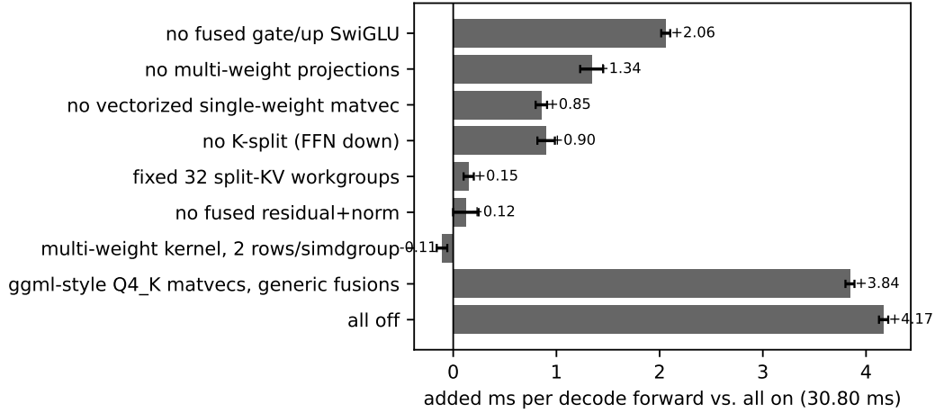
Figure 3: Leave-one-out effect of each switch on the decode step, in milliseconds per forward added relative to the all-on build; three runs each, error bars are the combined standard deviation. Table 8 in the appendix has the values.
