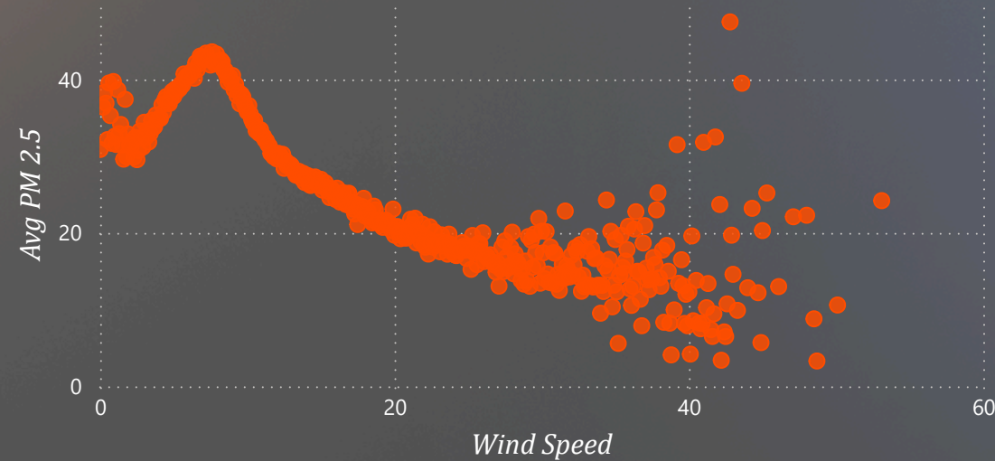
PM 2.5 by Wind Speed
