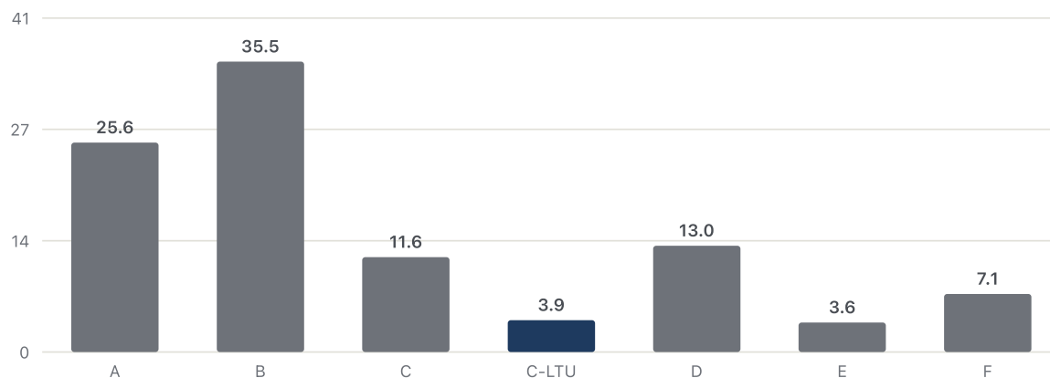
Figure 3. Greece's out-of-sample (leave-one-country-out) average residual, points, by model. C-LTU (highlighted) is the preferred specification. Corresponds to the out-of-sample column of Table 1.
