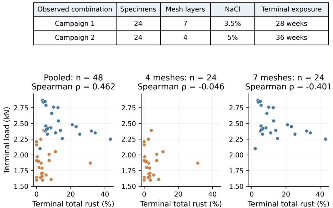
Figure 6.6: Campaign design and terminal surface-rust/load associations. The table shows the two observed combinations of mesh, chloride, and terminal exposure. Scatter plots use one terminal observation per specimen: pooled n = 48 , four-mesh n = 24 , seven-mesh n = 24 . Orange points are four-mesh specimens; blue points are seven-mesh specimens. Correlations are independently recomputed from the saved specimen summary. The pooled positive association does not establish an independent effect of rust on load.
