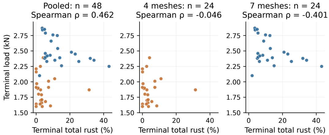
Figure 6.3: Campaign design and terminal surface-rust/load associations. The table shows the two observed combinations of mesh, chloride, and terminal exposure. Scatter plots use one terminal observation per specimen: pooled n = 48 , four-mesh n = 24 , seven-mesh n = 24 . Orange points are four-mesh specimens; blue points are seven-mesh specimens. Correlations are independently recomputed from the saved specimen summary. The pooled positive association does not establish an independent effect of rust on load.
