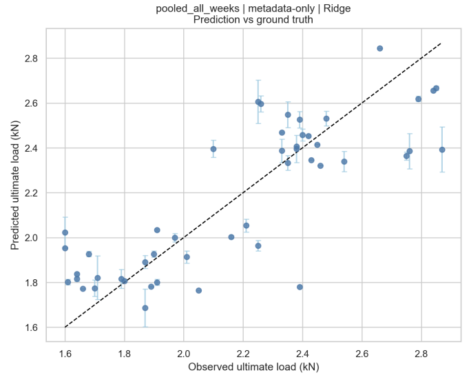
Fig. 4. Prediction-versus-ground-truth diagnostic for the metadata-only Ridge baseline in the main grouped evaluation. The dashed 1:1 line indicates perfect agreement between observed and predicted terminal load. The figure shows that the baseline follows the middle of the load range reasonably well but tends to overpredict the weakest specimens and underpredict the strongest ones, consistent with regression-to-the-mean behavior.
