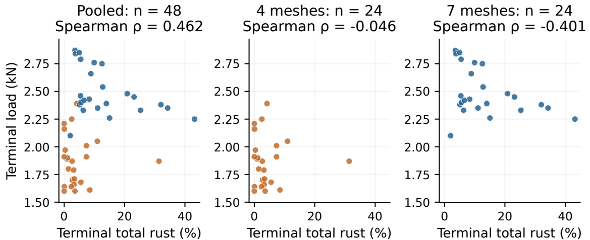
Figure 6.2: Campaign design and terminal surface-rust/load associations. The table shows the two observed combinations of mesh, chloride, and terminal exposure. Scatter plots use one terminal observation per specimen: pooled n = 48 , four-mesh n = 24 , seven-mesh n = 24 . Orange points are four-mesh specimens; blue points are seven-mesh specimens. Correlations are independently recomputed from the saved specimen summary. The pooled positive association does not establish an independent effect of rust on load.
