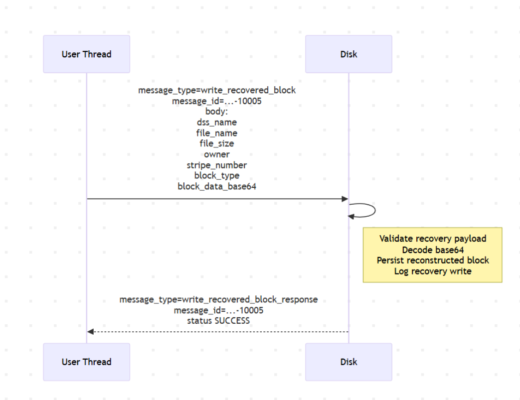
Figure 18: write_recovered_block to restore data after failure
