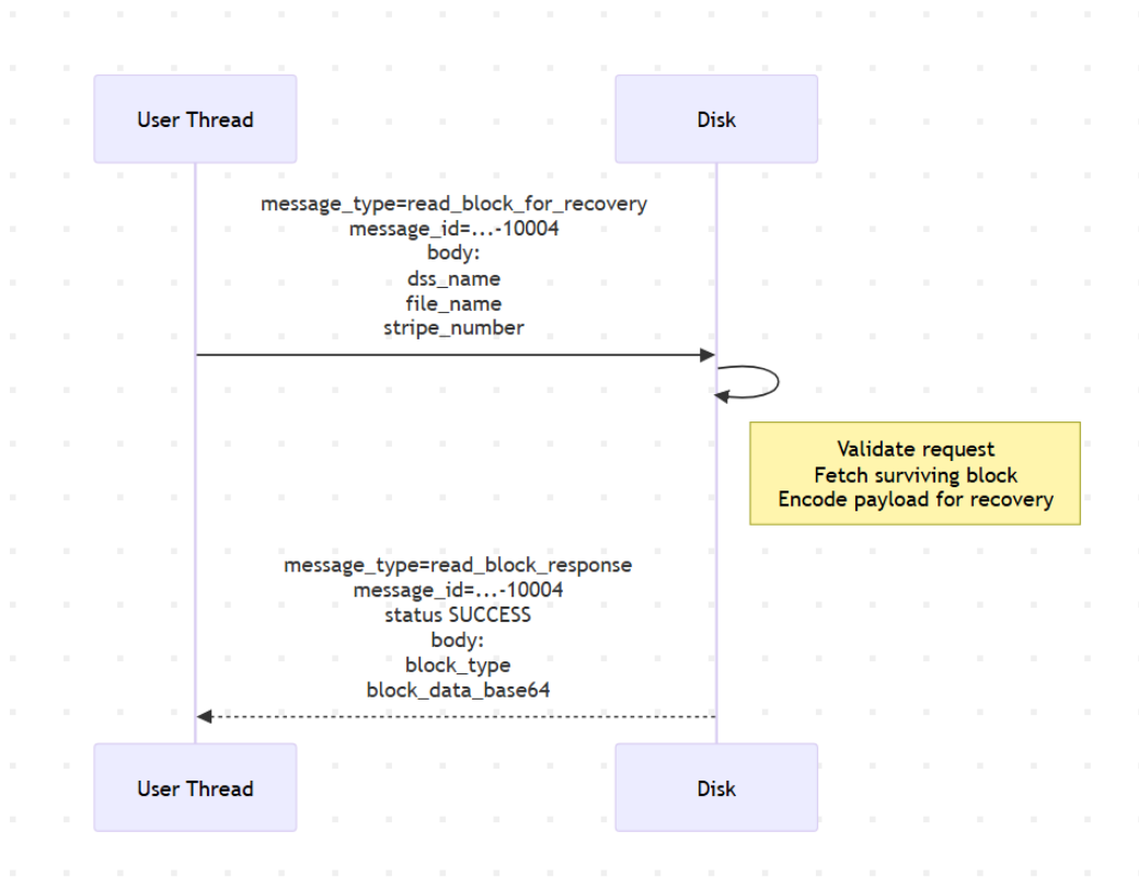
Figure 17: read_block_for_recovery during reconstruction
