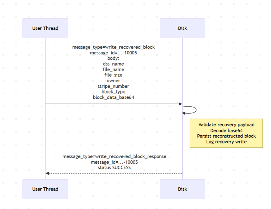
Figure 18: write_recovered_block to restore data after failure
