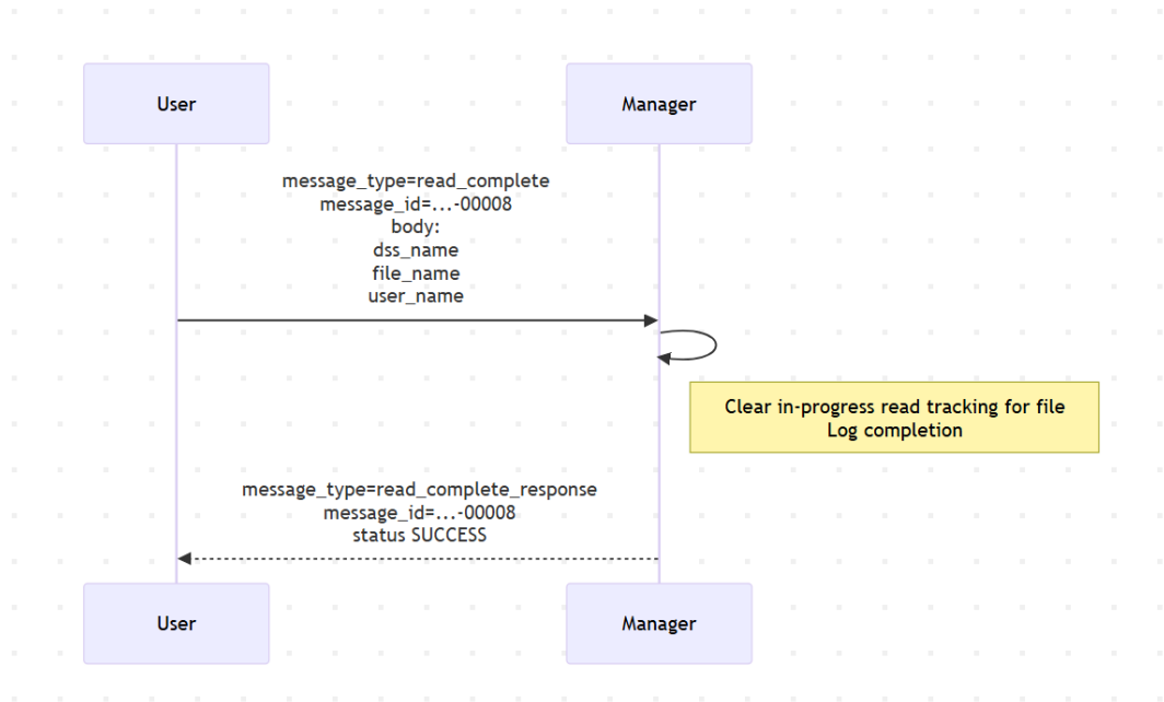
Figure 8: read_complete : clearing in-progress tracking
