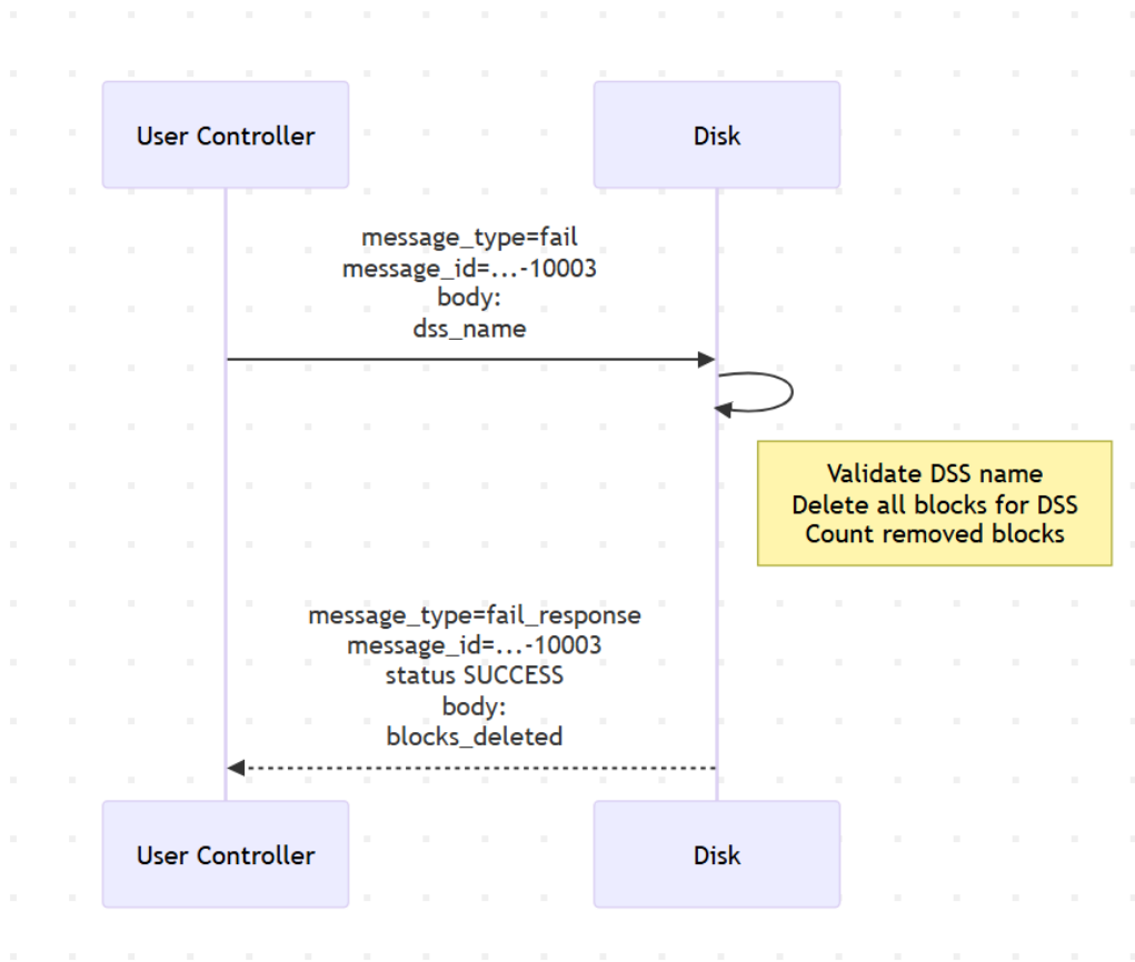
Figure 16: User-initiated fail to simulate a disk crash
