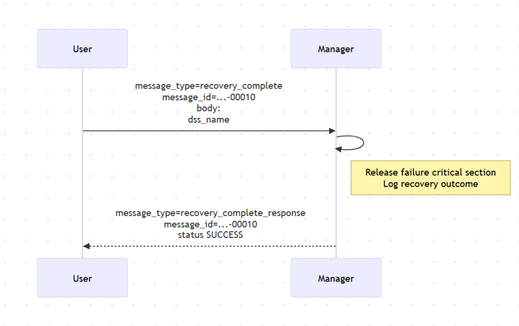
Figure 10: recovery_complete : leaving the failure critical section
