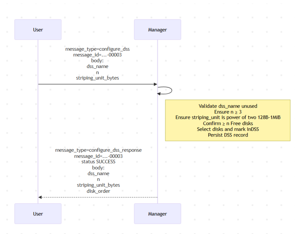
Figure 3: configure_dss validation and response flow
