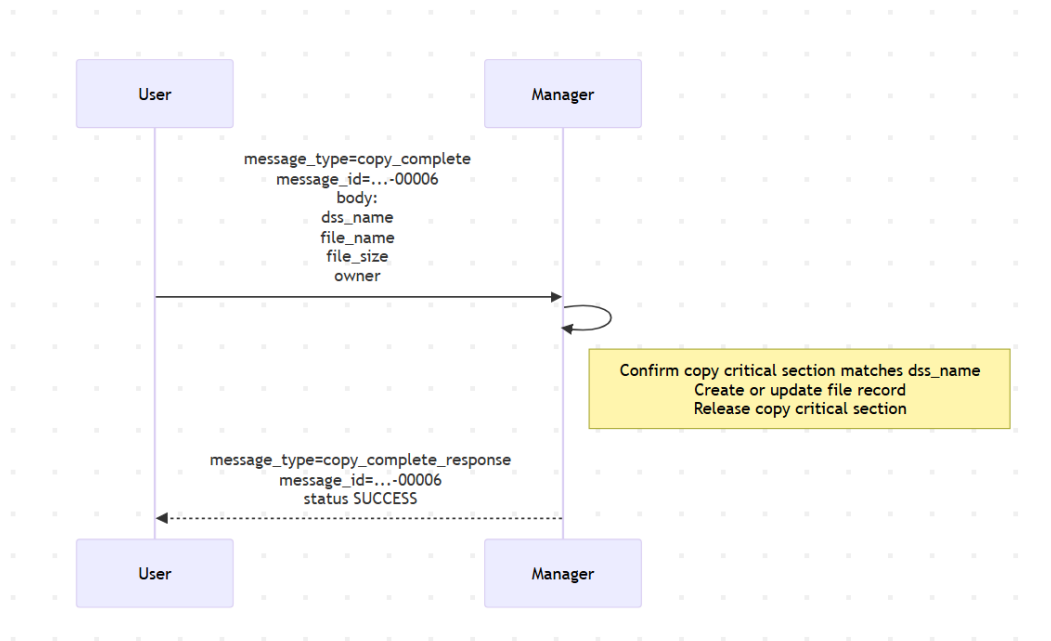
Figure 6: Copy phase 2: recording file metadata and releasing the critical section
