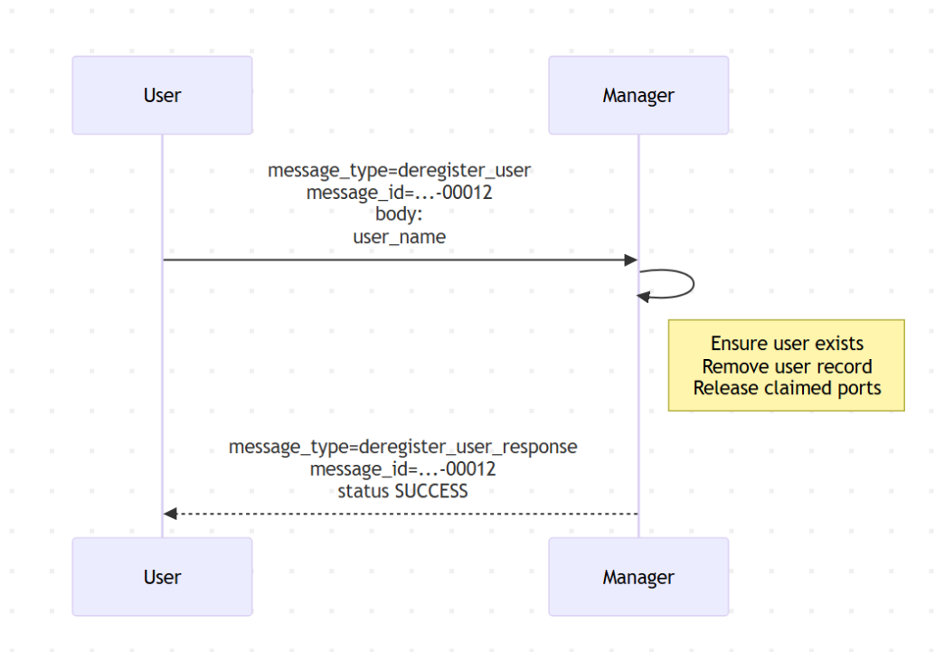
Figure 12: Manager happy path for deregister_user
