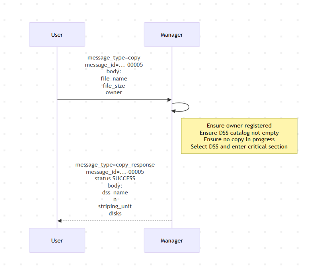
Figure 5: Copy phase 1: entering the critical section and returning DSS endpoints
