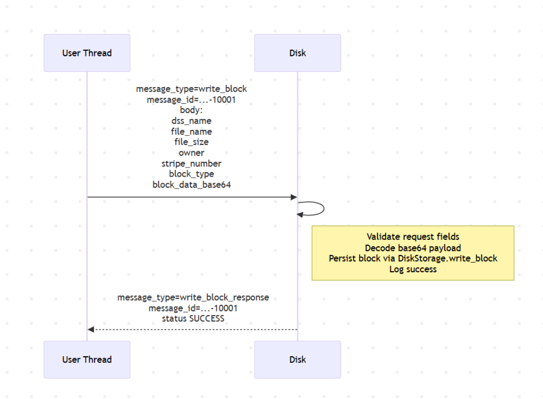
Figure 14: User to disk write_block
