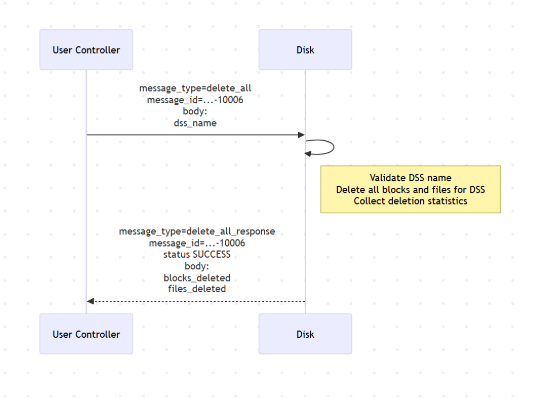
Figure 19: delete_all for DSS decommissioning cleanup
