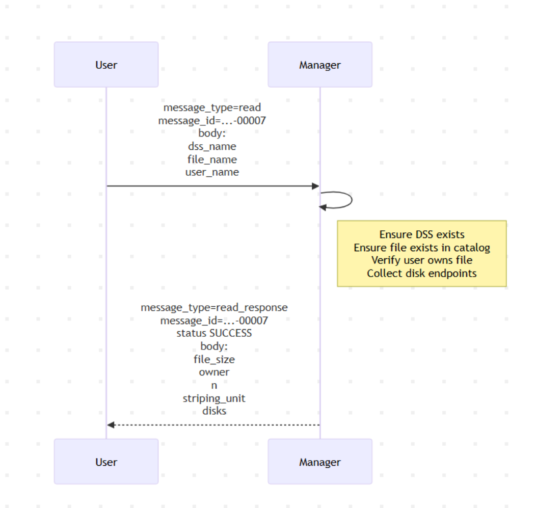
Figure 7: read phase 1: returning disk endpoints with ownership checks
