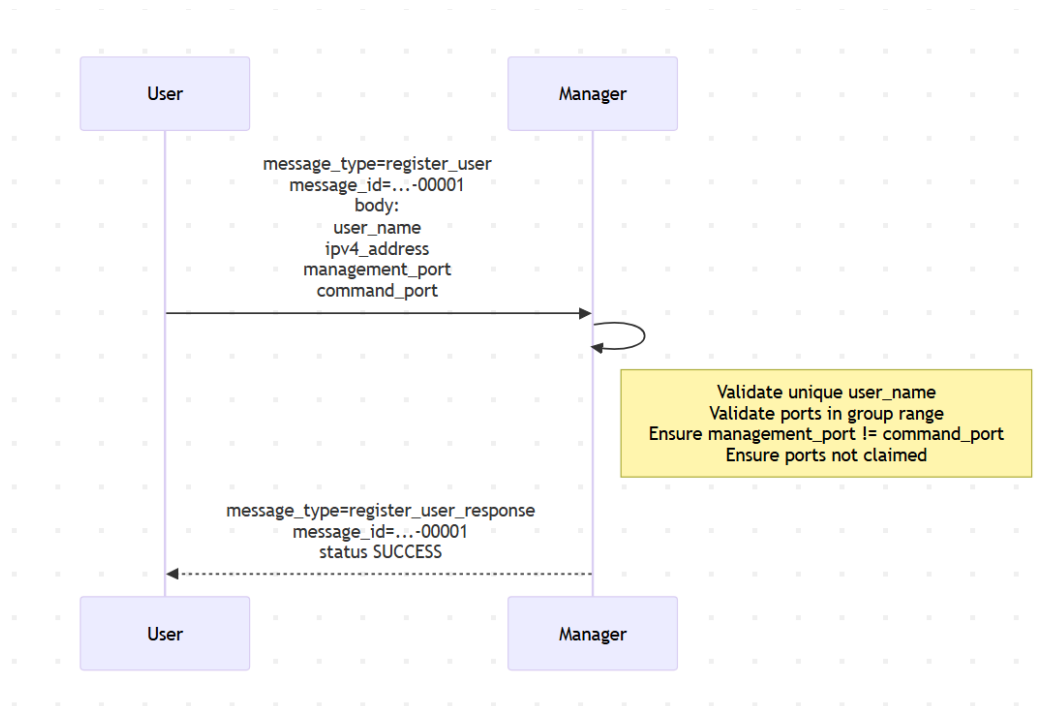
Figure 1: Manager happy path for register_user
