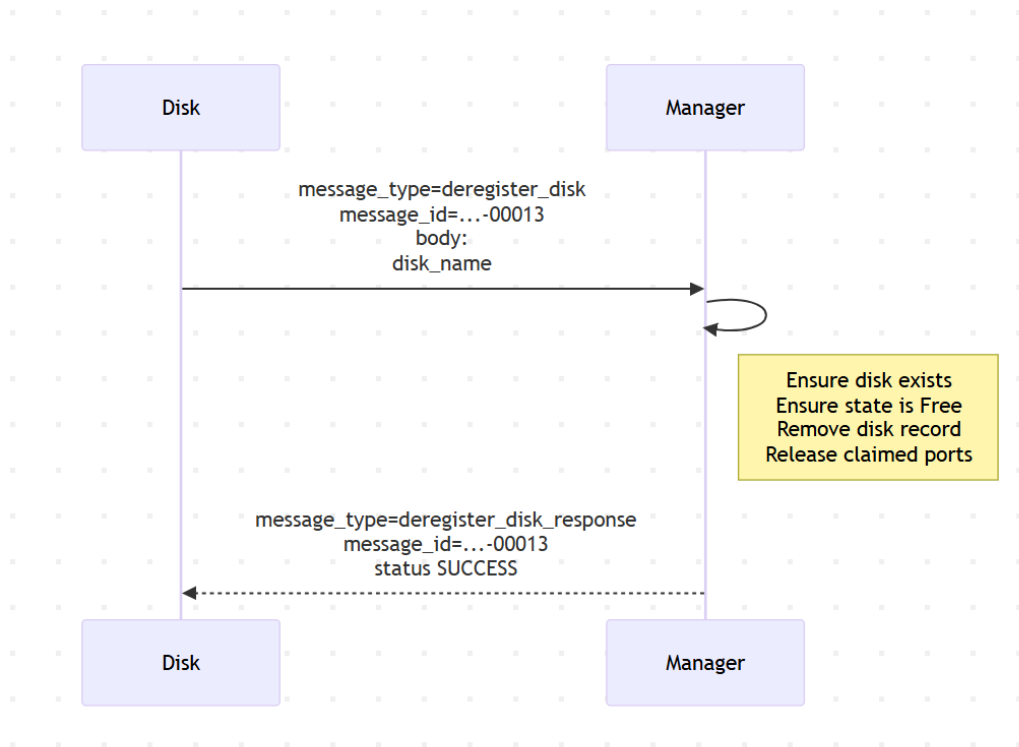
Figure 13: Manager happy path for deregister_disk
