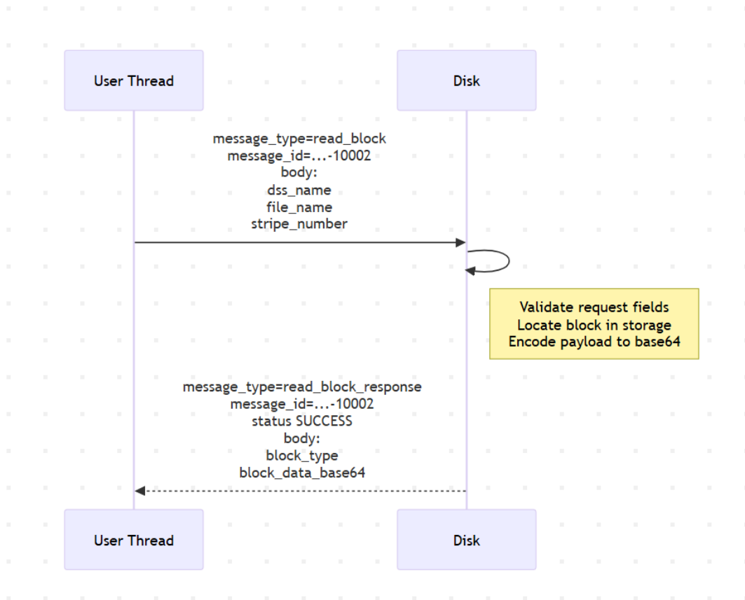
Figure 15: User to disk read_block
