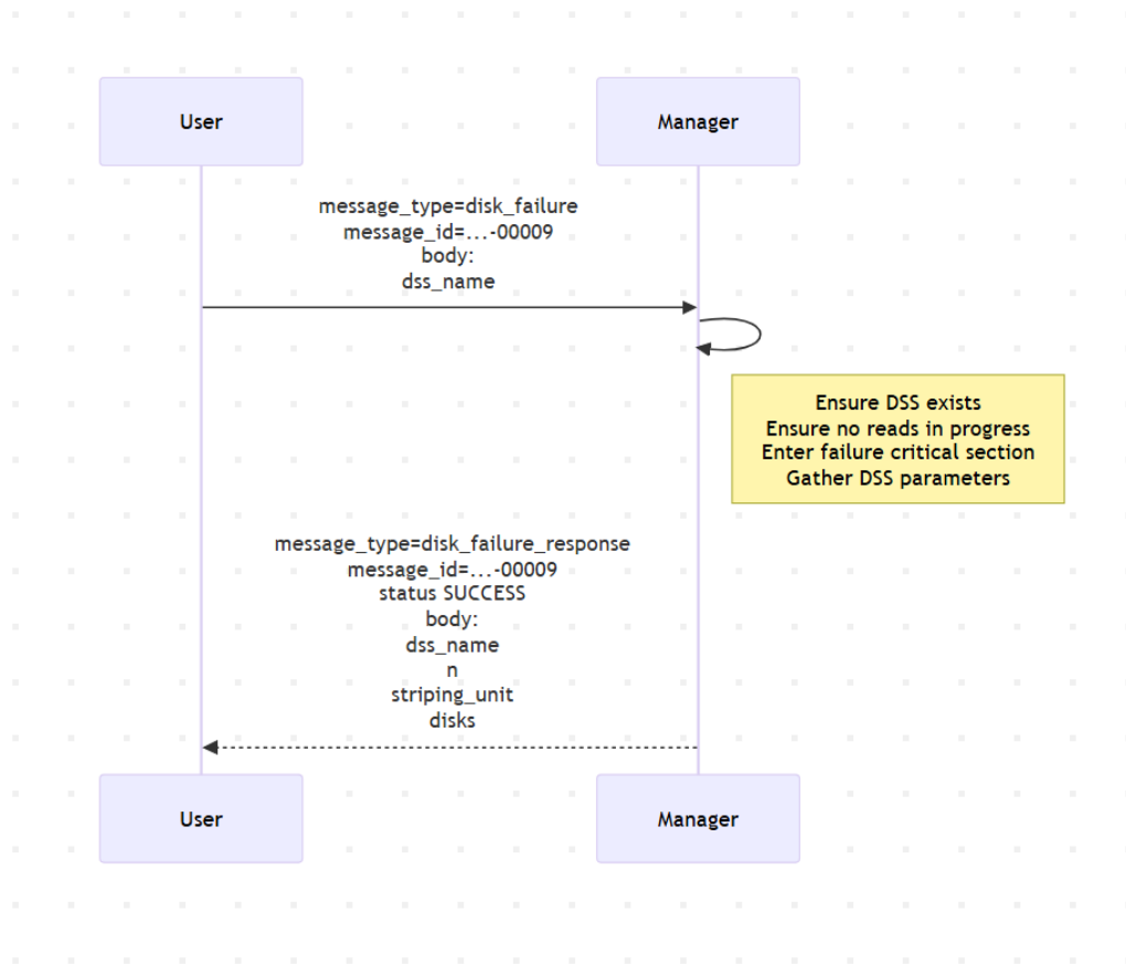
Figure 9: disk_failure phase 1: entering the failure critical section
