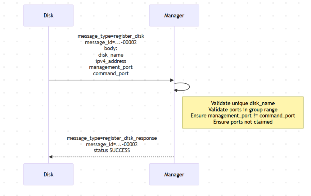
Figure 2: Manager happy path for register_disk
