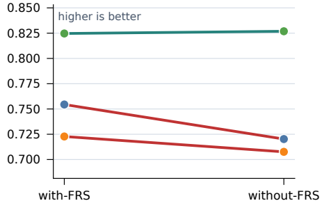
Accuracy
