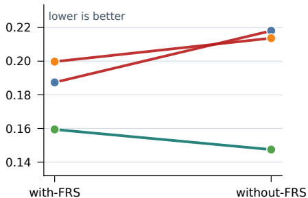
Brier score
