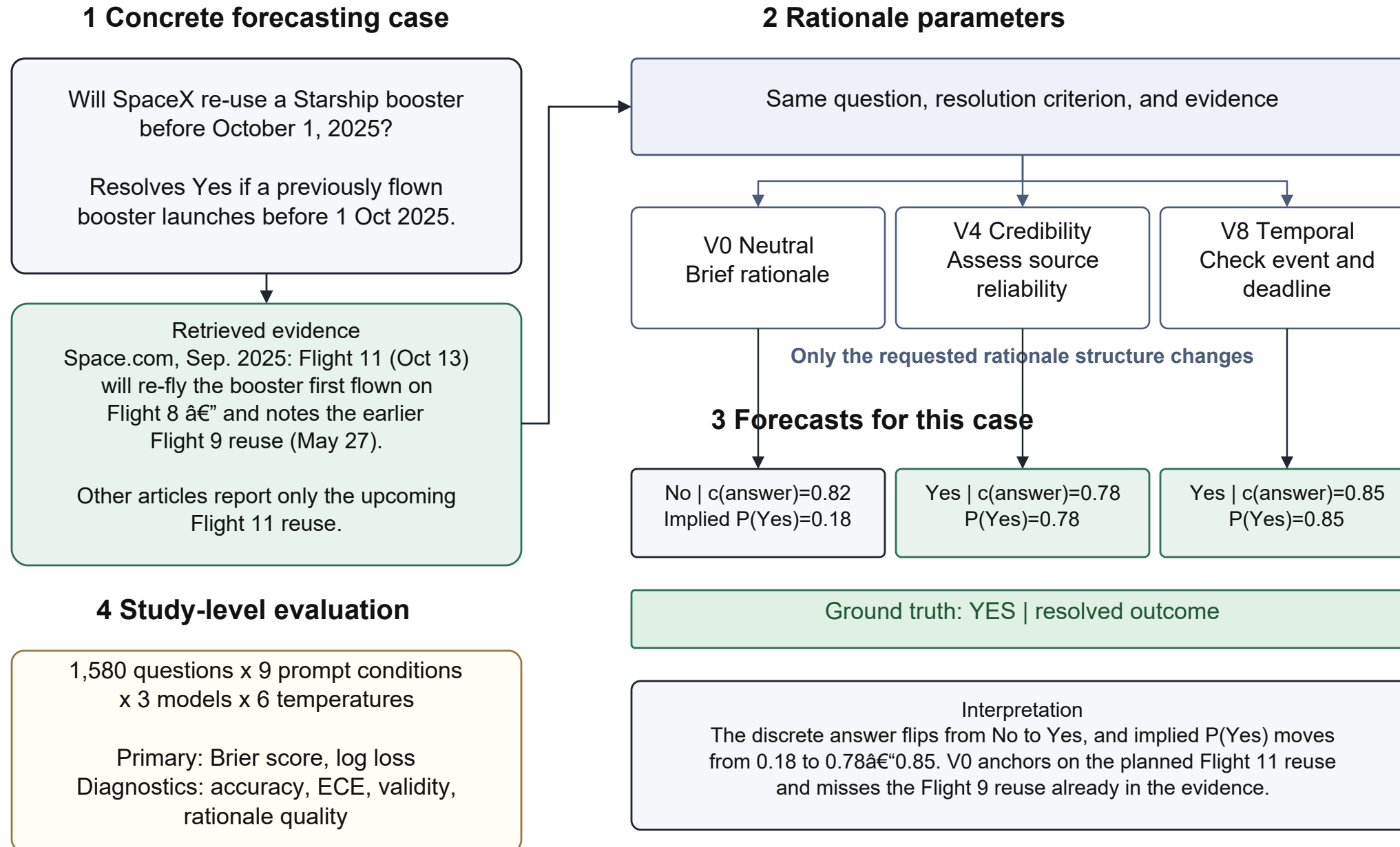
Figure 1: Representative case from the forecasting study (Metaculus 29222; GPT-OSS-120B, T=0.75). Boxes reproduce the raw answer and the confidence in that answer, c(\text{answer}) . For evaluation, No forecasts are converted using P(\text{Yes}) = 1 - c(\text{answer}) . Accuracy uses the discrete answer, whereas Brier score and log loss use the implied P(\text{Yes}) . The example is illustrative; the paper's main claims are based on paired aggregate evaluation.
