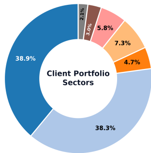
Client Portfolio
